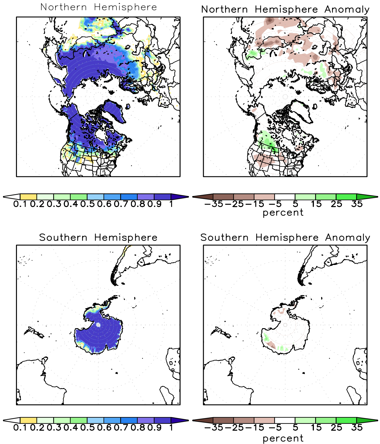
FIGURE A2.2. SSM/I derived snow cover frequency (%) (left) and snow cover anomaly (%) (right) for the month of MAR 2009 based on 1987 - 2006 base period for the Northern Hemisphere (top) and Southern Hemisphere (bottom). It is generated using the algorithm described by Ferraro et. al, 1996, Bull. Amer. Meteor. Soc., vol 77, 891-905.
