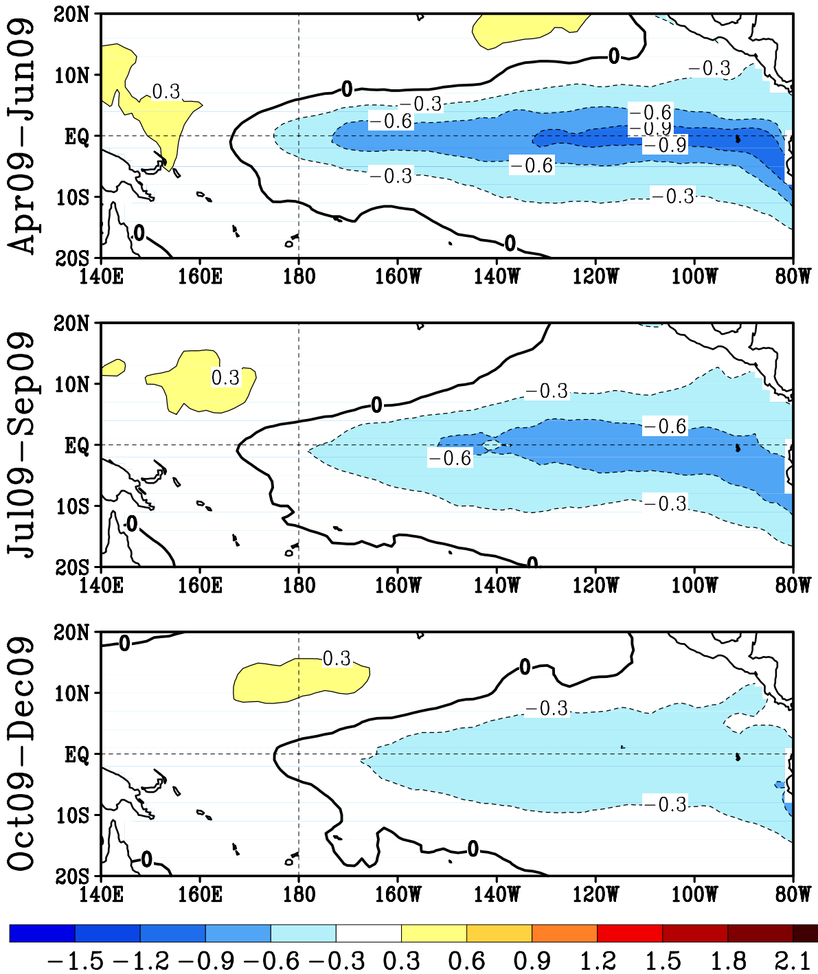
FIGURE F5. Predicted 3-month average sea surface temperature anomalies from the NCEP/CPC Markov model (Xue et al. 2000, J. Climate , 13 , 849-871). The forecast is initiated in MAR 2009. Contour interval is 0.3C and negative anomalies are indicated by dashed contours. Anomalies are calculated relative to the 1971-2000 climatology.
