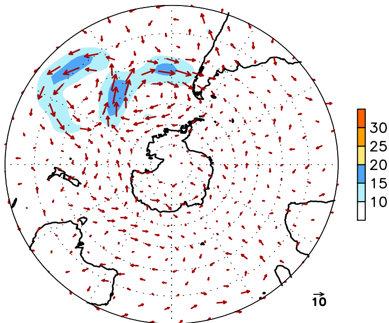
FIGURE E16. Southern Hemisphere mean (left) and anomalous (right) 300-hPa vector wind (CDAS/Reanalysis) for MAR 2009. Mean (anomaly) isotach contour interval is 10 (5) \text{ms}^{-1} . Values greater than 30 \text{ms}^{-1} (left) and 10 \text{ms}^{-1} (rights) are shaded. Anomalies are departures from the 1979-95 base period monthly means.
