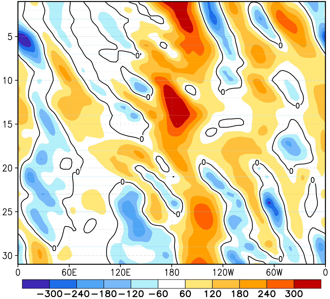
FIGURE E12. Northern Hemisphere: Daily 500-hPa height anomalies for MAR 2009 averaged over the 5° latitude band centered on 40°N. Positive values are indicated by solid contours and dark shading. Negative values are indicated by dashed contours and light shading. Contour interval is 60 m. Anomalies are departures from the 1979-95 base period daily means.
