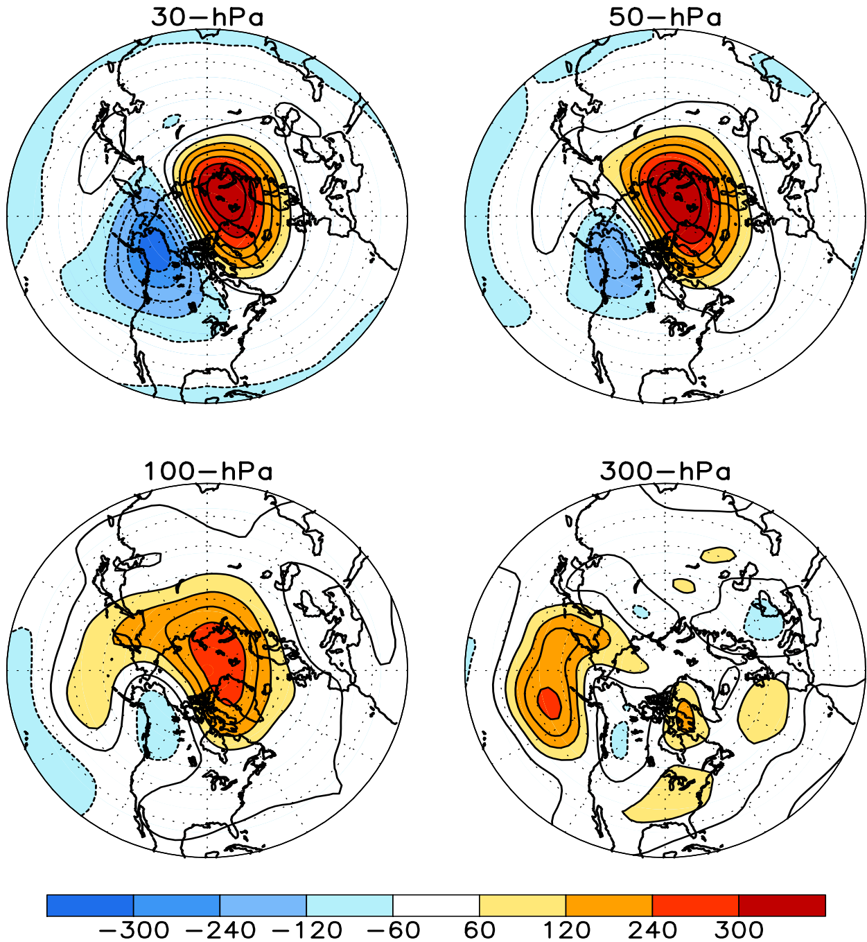
FIGURE S1. Stratospheric height anomalies (m) at selected levels for MAR 2009. Positive values are indicated by solid contours and dark shading. Negative values are indicated by dashed contours and light shading. Contour interval is 60 m. Anomalies are calculated from the 1979–95 base period means. Winter Hemisphere is shown.
