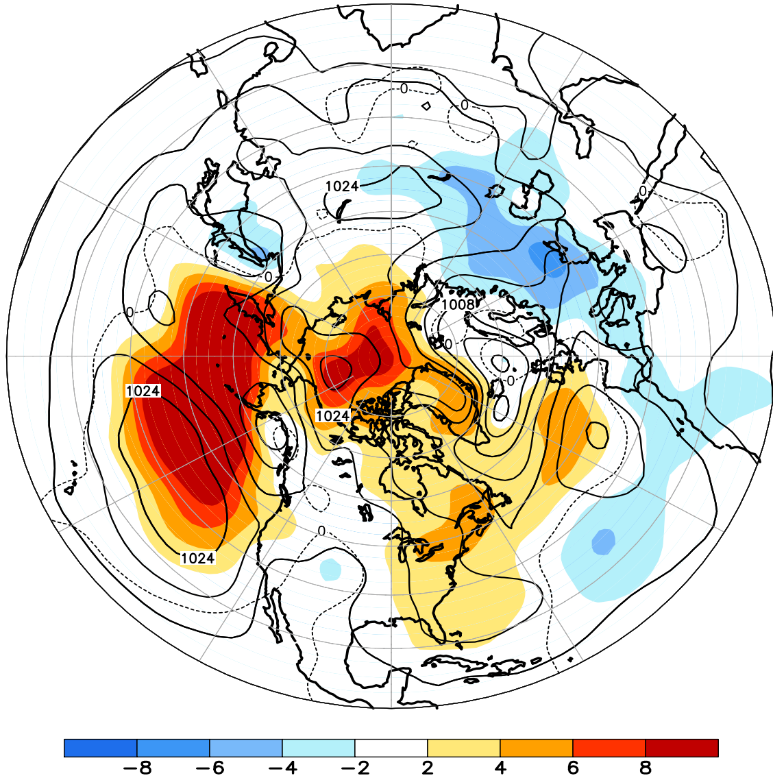
FIGURE E8. Northern Hemisphere mean and anomalous sea level pressure (CDAS/Reanalysis) for MAR 2009. Mean values are denoted by solid contours drawn at an interval of 4 hPa. Anomaly contour interval is 2 hPa with values less (greater) than -2 hPa (2 hPa) indicated by dark (light) shading. Anomalies are calculated as departures from the 1979-95 base period monthly means.
