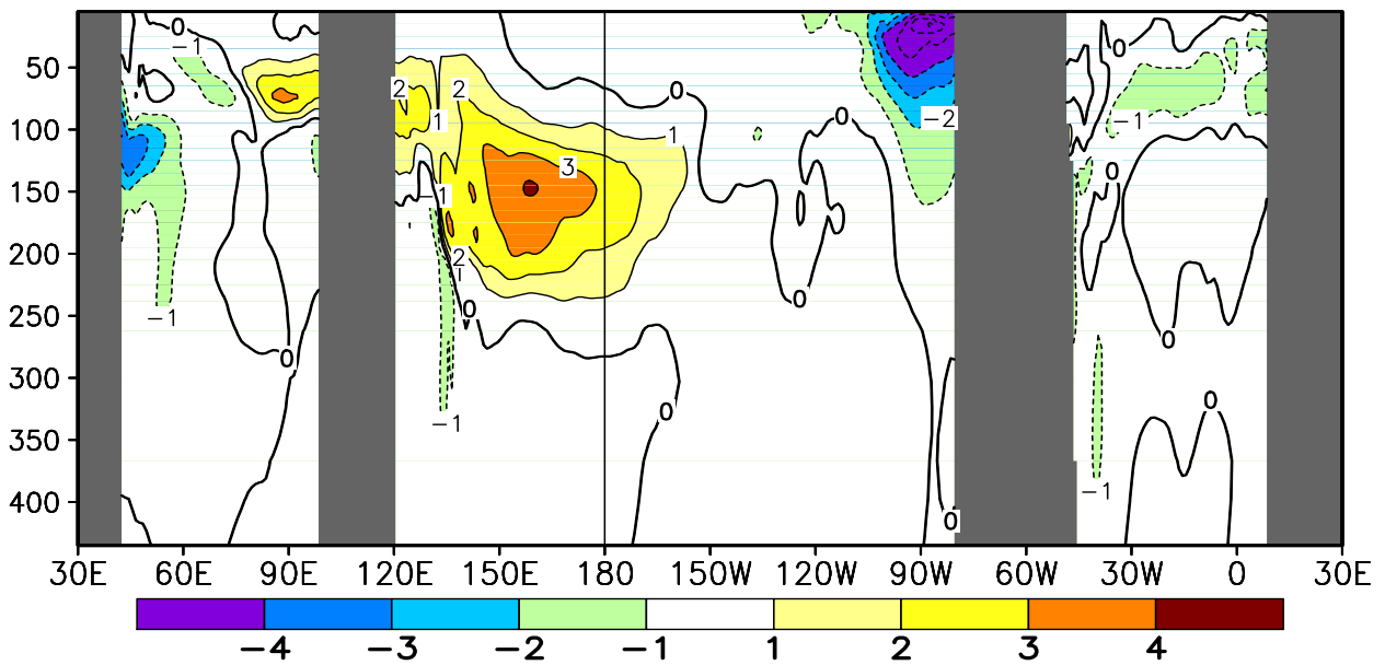
FIGURE T17. Equatorial depth–longitude section of ocean temperature (top) and ocean temperature anomalies (bottom) for MAR 2009. Contour interval is 1°C. Dashed contours in bottom panel indicate negative anomalies. Data are derived from the NCEP’s global ocean data assimilation system version 2 which assimilates oceanic observations into an oceanic GCM (Xue, Y. and Behringer, D.W., 2006: Operational global ocean data assimilation system at NCEP, to be submitted to BAMS). Anomalies are departures from the 1982–2004 base period means.
