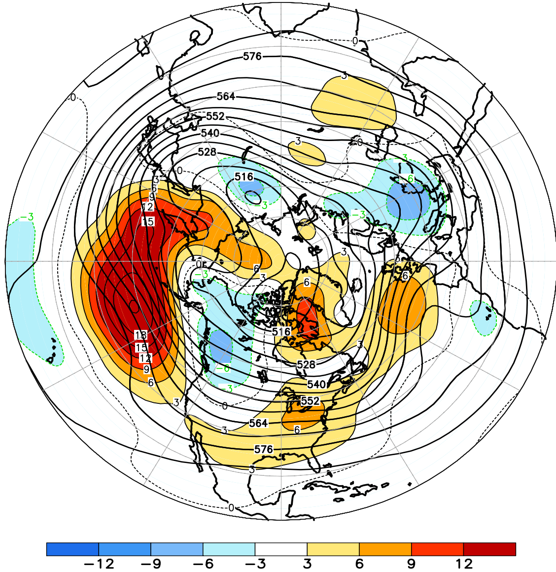
FIGURE E9. Northern Hemisphere mean and anomalous 500-hPa geopotential height (CDAS/Reanalysis) for MAR 2009. Mean heights are denoted by solid contours drawn at an interval of 6 dam. Anomaly contour interval is 3 dam with values less (greater) than -3 dam (3 dam) indicated by dark (light) shading. Anomalies are calculated as departures from the 1979-95 base period monthly means.
