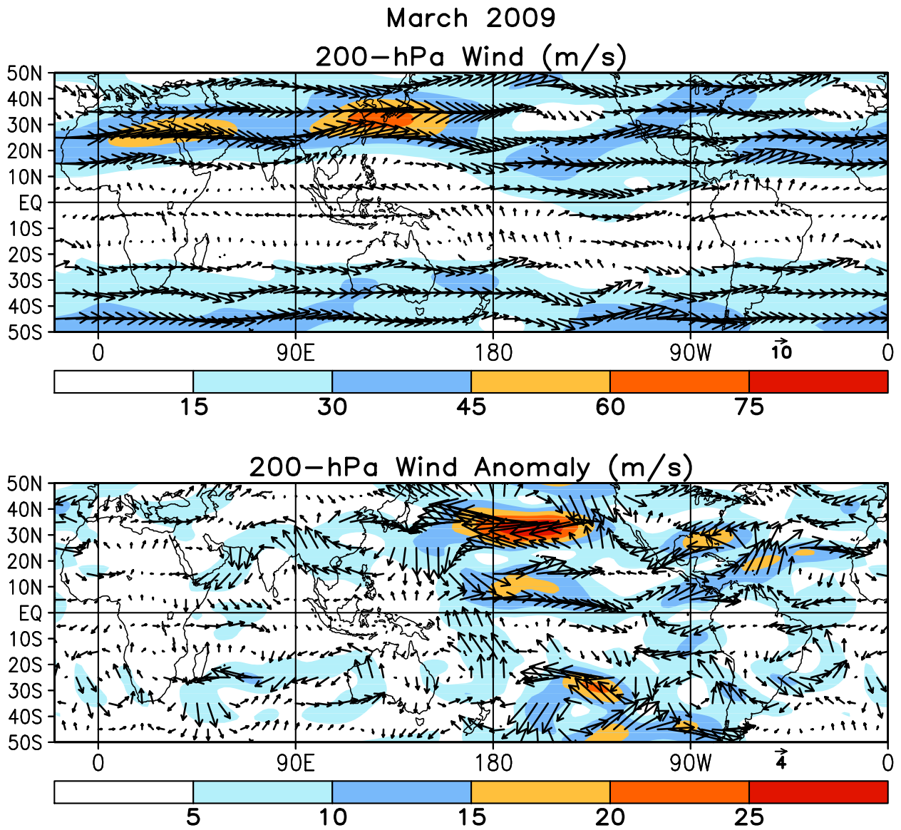
FIGURE T21. Mean (top) and anomalous (bottom) 200-hPa vector wind (CDAS/Reanalysis) for MAR 2009. Contour interval for isotachs is 15 \text{ ms}^{-1} (top) and 5 \text{ ms}^{-1} (bottom). Anomalies are departures from 1979–95 base period monthly means.
