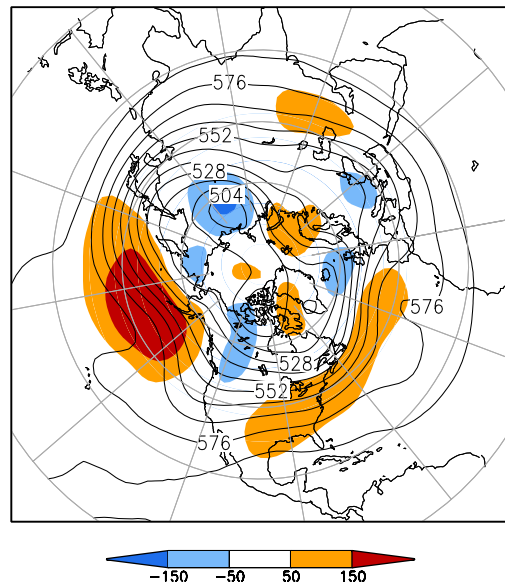
500-hPa Height (dm) & Anomalies (m) (Mar 1–15, 2009)
