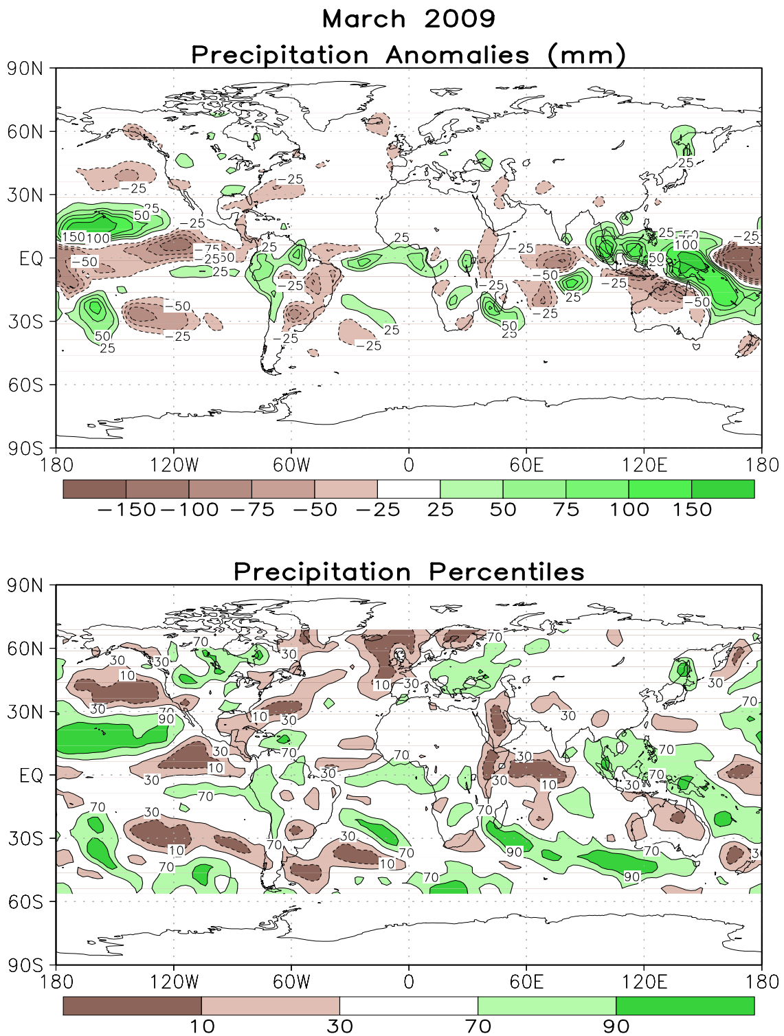
FIGURE E3. Anomalous precipitation (mm, top) and precipitation percentiles based on a Gamma distribution fit to the 1979–2000 base period data (bottom) for MAR 2009. Data are obtained from a merge of raingauge observations and satellite-derived precipitation estimates (Janowiak and Xie 1999, J. Climate , 12 , 3335–3342). Contours are drawn at 200, 100, 50, 25, -25, -50, -100, and -200 mm in top panel. Percentiles are not plotted in regions where mean monthly precipitation is <5mm/month.
