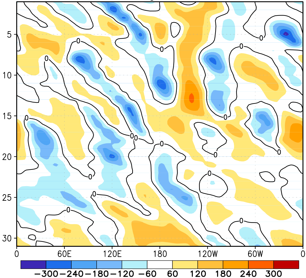
FIGURE E18. Southern Hemisphere: Daily 500-hPa height anomalies for MAR 2009 averaged over the 5° latitude band centered on 40°S. Positive values are indicated by solid contours and dark shading. Negative values are indicated by dashed contours and light shading. Contour interval is 60 m. Anomalies are departures from the 1979-95 base period daily means.
