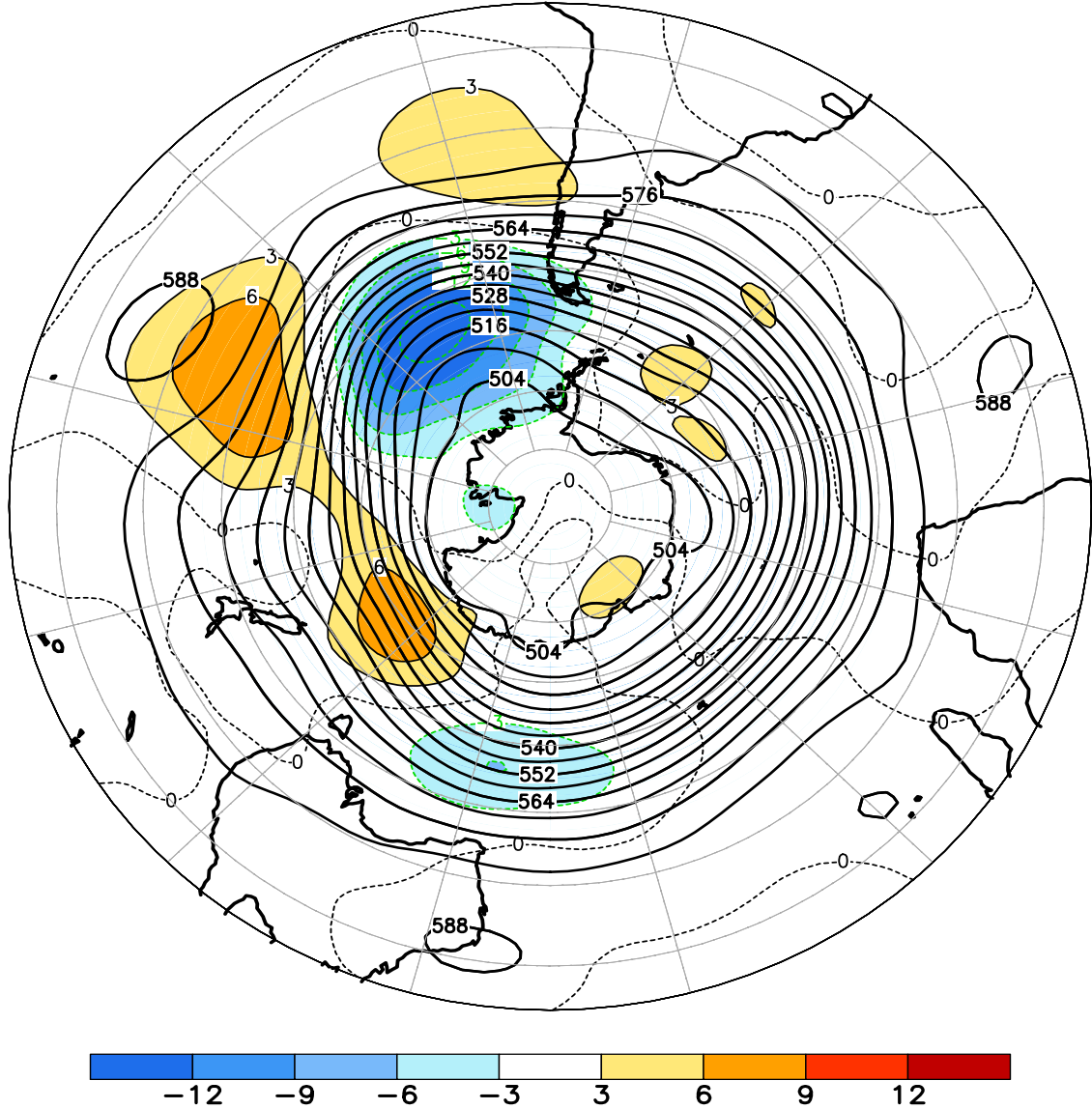
FIGURE E15. Southern Hemisphere mean and anomalous 500-hPa geopotential height (CDAS/Reanalysis) for MAR 2009. Mean heights are denoted by solid contours drawn at an interval of 6 dam. Anomaly contour interval is 3 dam with values less (greater) than -3 dam (3 dam) indicated by dark (light) shading. Anomalies are calculated as departures from the 1979-95 base period monthly means.
