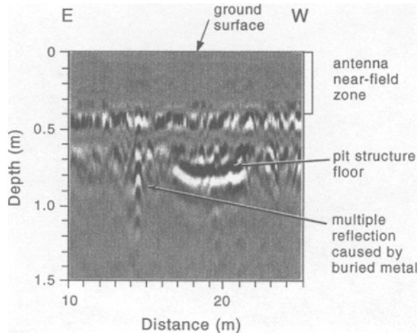
Figure 3. Ground-penetrating radar profile of a pit structure, Valencia site, Arizona. Vertical exaggeration 10:1.
