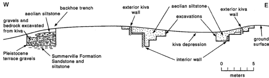
Figure 6. Cross section of the Bluff Great House site great kiva and the test trench to the west showing the stratigraphy and archaeological features visible in GPR maps.
