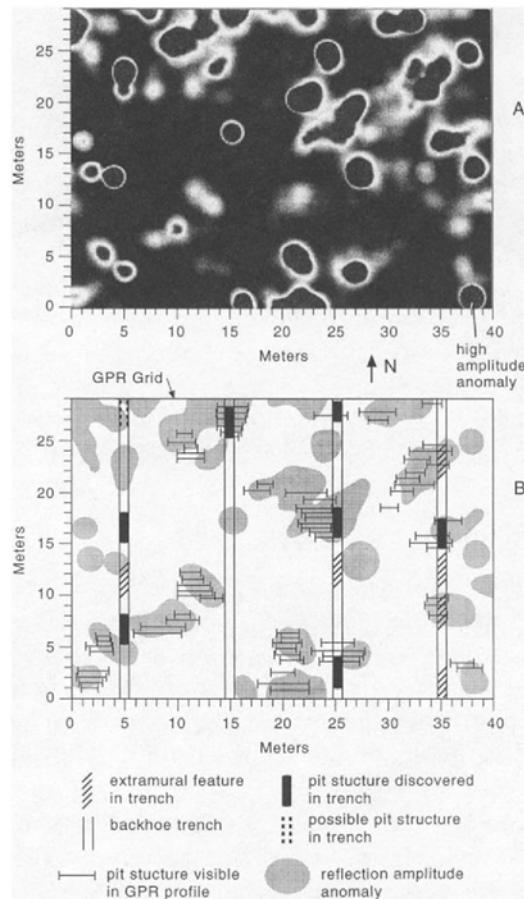
Figure 4. Amplitude anomaly map and interpretation, Valencia site, Arizona. Map A is the spatial distribution of high amplitude radar reflections in a slice from 50 to 100 cm below the surface. Map B is an overlay of these amplitude anomalies and the location of the pit structures visible in individual profiles. These are compared to the features that were visible in backhoe trenches.
