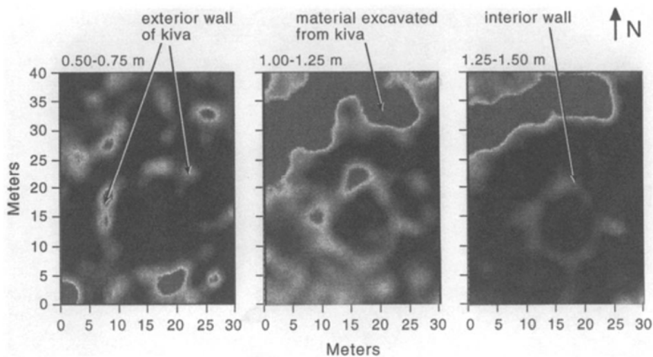
Figure 7. Amplitude slice-maps of processed 500 MHz GPR data from the Bluff Great House site great kiva. Each slice is analogous to an arbitrary excavation level, except the GPR maps show relative radar reflection amplitudes from buried features instead of the features themselves.
