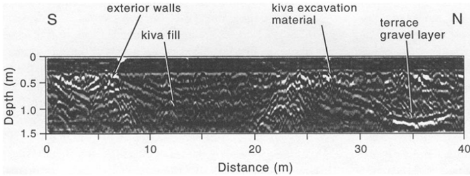
Figure 8. Two-dimensional GPR profile of the Bluff Great House site great kiva. Vertical exaggeration 5:1.
