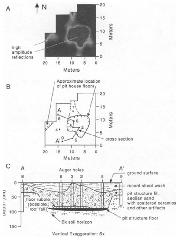
Figure 5. Southwest Bluff site maps and cross section. Map A is the spatial distribution of high amplitude reflections in the slice from 80 to 110 cm below the surface. The auger holes and cross-section location, with the outline of the pit structure floor are shown in B. The cross-section (C) shows the location of the pit structure floor and pit fill.
