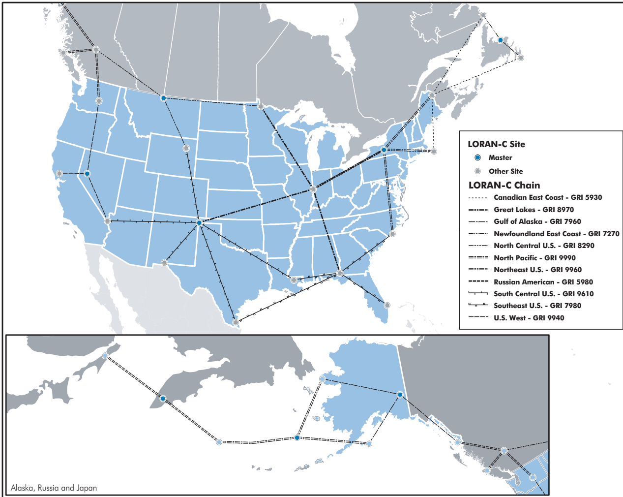
Figure 3-3: LORAN-C Chains
