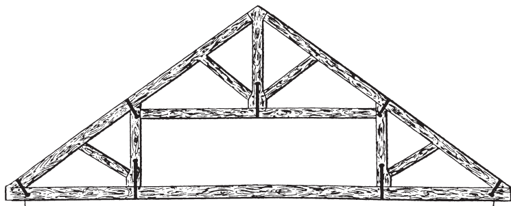
Fig. 1. Kingpost truss superimposed above queenpost truss, from Plate I of Francis Price, The British Carpenter , 1733.
