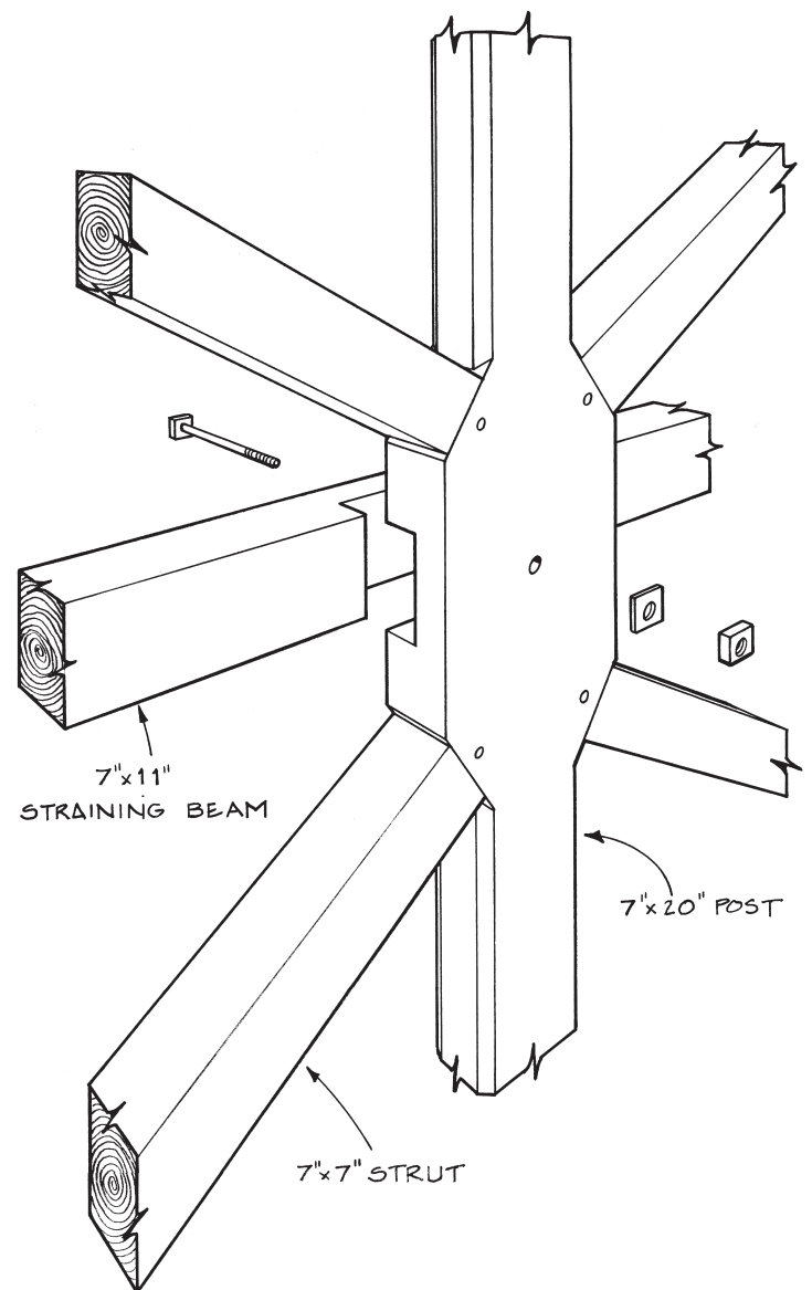
Fig. 5. Central Moravian 7x20 oak kingpost, accommodating struts in four directions and the halved crossing of a straining beam.
