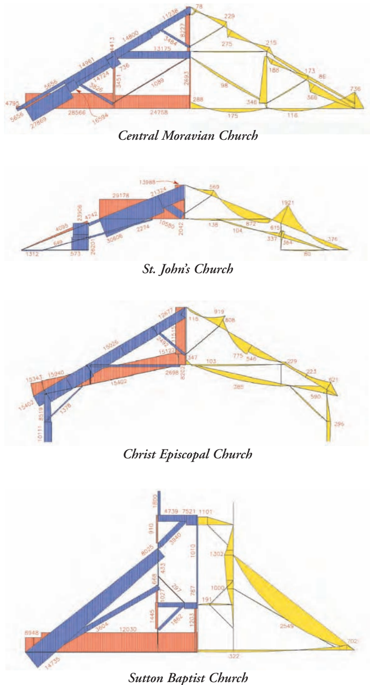
Fig. 1. In the diagrams above (not to scale), axial forces are on the left (blue for compression, red for tension, in lbs.) and bending stresses (yellow, in lbs.) are on the right.
