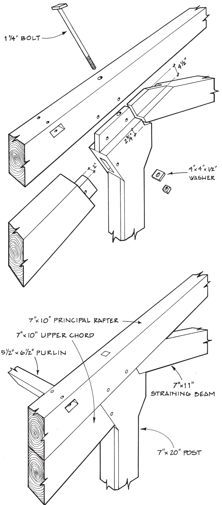
Fig. 7. Exploded and assembled views of queenpost head, showing elements of queenpost truss captured by principal rafter of kingpost truss.
