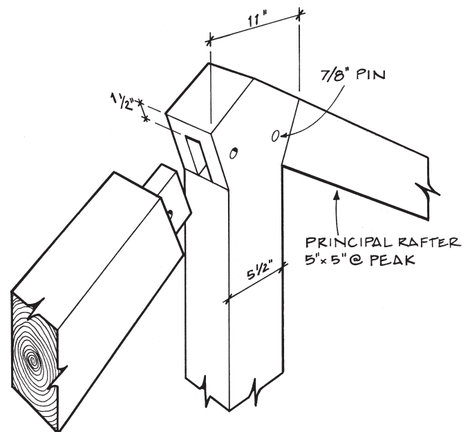
Fig. 15. Detail at Christ Episcopal kingpost head.
