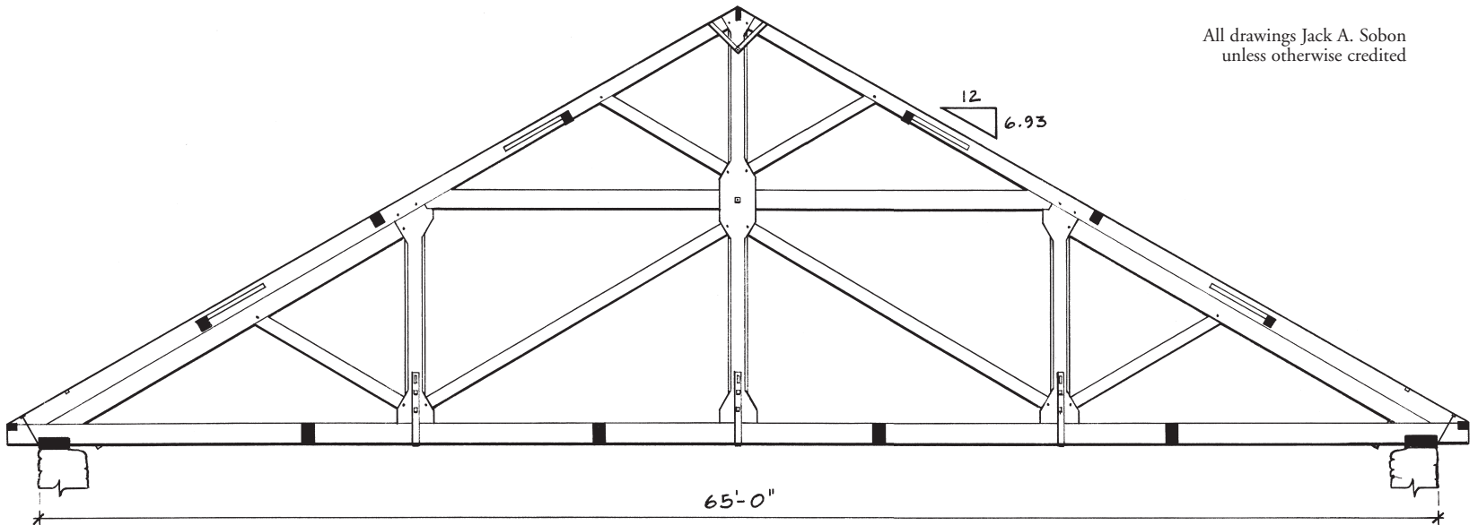
Fig. 4. Composite truss at Central Moravian Church, Bethlehem, Pa. (1803-1806). Kingpost and queenpost elements interact.
