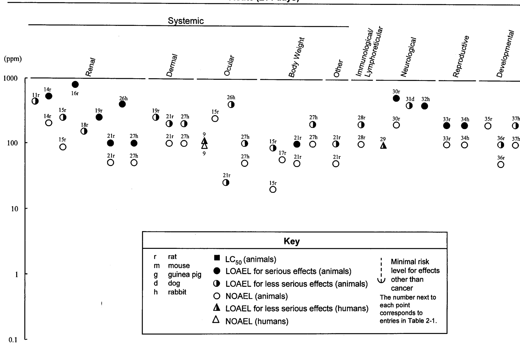
Figure 2-1. Levels of Significant Exposure to 2-Butoxyethanol - Inhalation (cont.)
