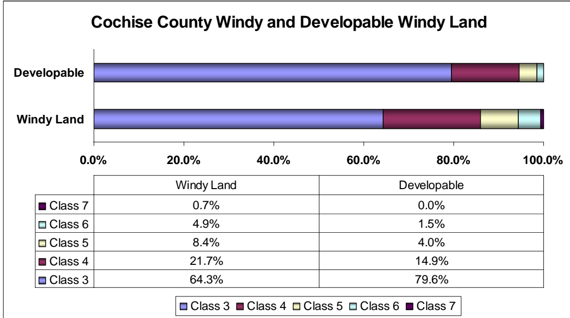
Figure 4 Windy Land by Wind Class for Cochise County
