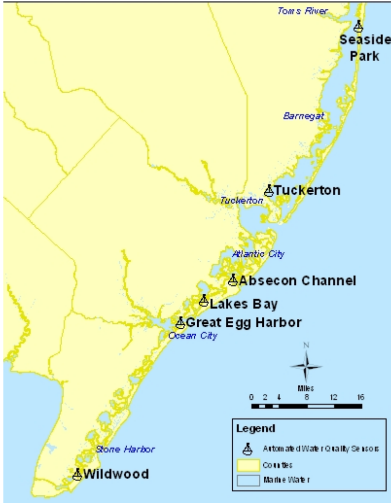
Figure 5. Automated Data-logger Monitoring Locations in New Jersey's Buoy Monitoring Network.
