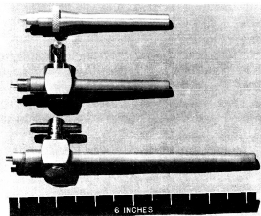
Figure 12. - Evolution of the contingency-feeding-system valve-adapter pontube (earliest concept at top, intermediate concept at center, and current design at bottom).
