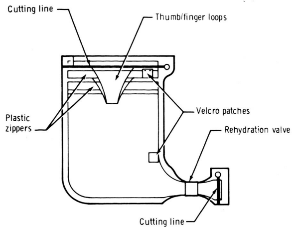
Figure 20. - Rehydratable-food spoon-bowl package.
