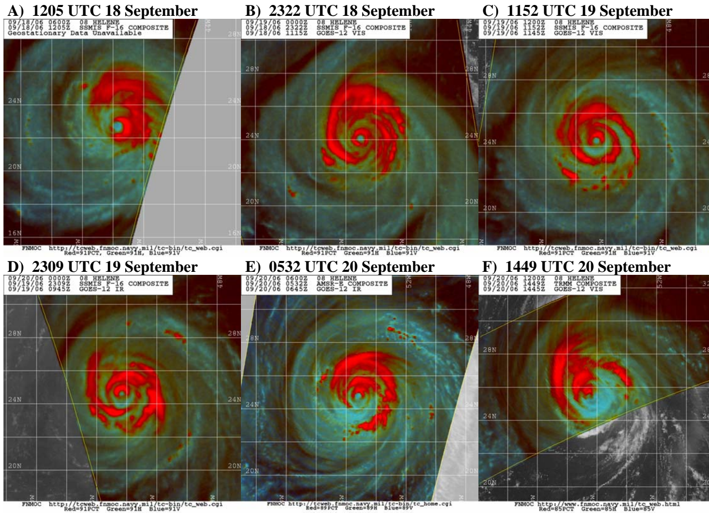
Figure 4. Series f composite 85-91 GHz passive microwave images of Hurricane Helene during 18-20 September 2006. Images courtesy of the Fleet Numerical Meteorology and Oceanography Center (FNMOC).
