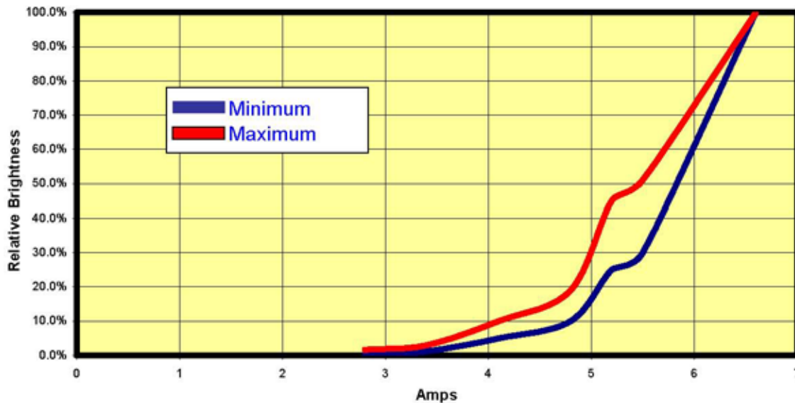
Figure 1: Dimming Curve
