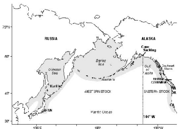
Figure 1. Steller Sea Lion Distribution
