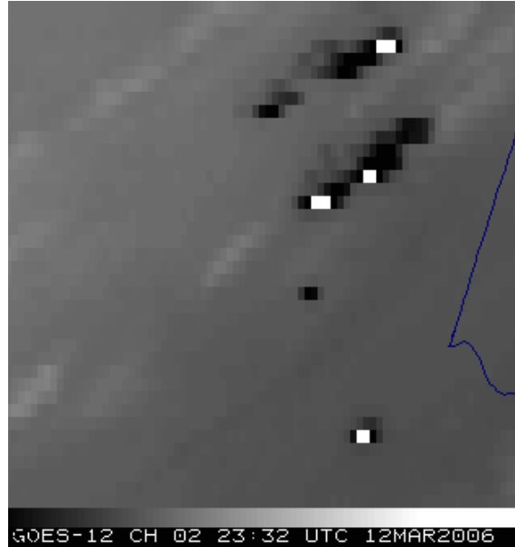
Figure 1: Example of rollover in observations by GOES-12 Imager Channel 2. The image contains an area of fires with brightness temperatures sometimes exceeding 342K. The higher the GVAR count value, the blacker the pixel. However, the observations in the hottest regions exceed the GVAR maximum and have rolled over to low values, producing the white pixels. The irregular blue line on the right is a portion of a state border superimposed on the image. (Figure courtesy of Scott Bachmeier, Space Science and Engineering Center, University of Wisconsin, Madison, WI)
