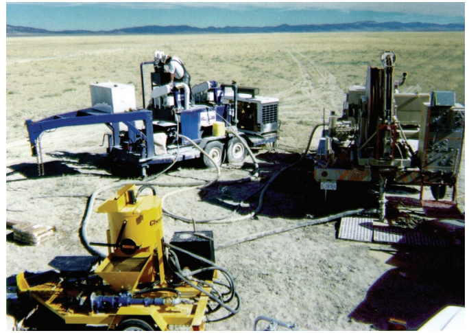
The microhole drilling system is shown here in central Nevada drilling cased 1.25-inch diameter microholes for emplacement of seismic instrumentation. The tan equipment (right) is the coiled tube drilling rig, the blue is a mud conditioning system, and the yellow is a PVC casing grouting system.
