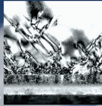
Transmission electron micrograph showing a cross-section of ACSi film and underlying buffer layers on metal tape.
