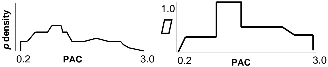
Figure 2. pdf for the tests and \square -df for the models (PAC is in 10^3 g's).
