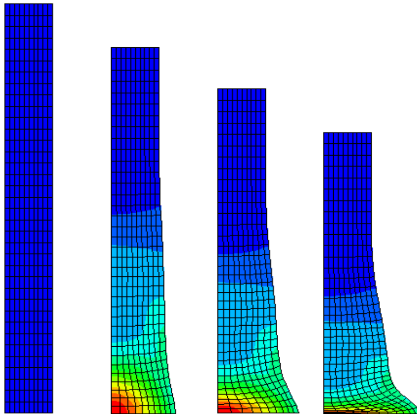
Figure 4. Simulation of the Taylor test described in the text. The figures show the half-cylinder shapes at times of 0 \mu s, 17 \mu s, 33 \mu s, and 50 \mu s after impact (from left to right).
