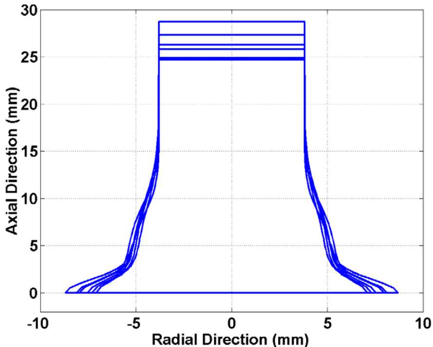
Figure 5. Six representative Taylor-test profiles for the steel cylinder predicted in a short Monte Carlo run in which there is a high degree of uncertainty in its plastic behavior. The
