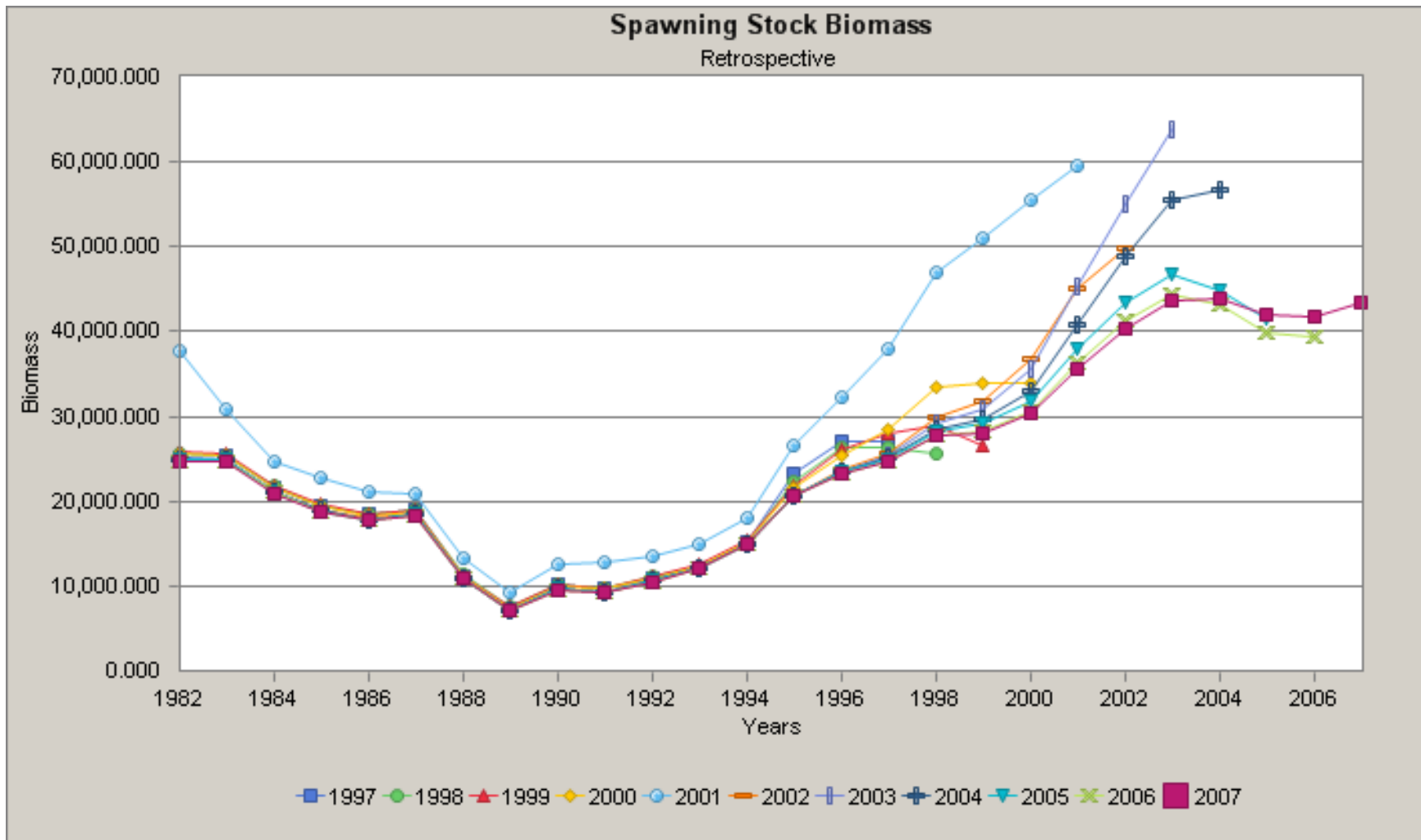
Figure A5. Retrospective analysis of spawning stock biomass (metric tons) for summer flounder.
