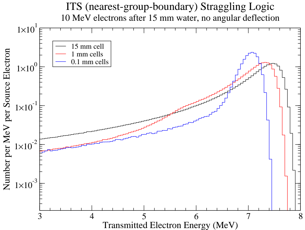
Figure 2. Results of the nearest-group-boundary straggling logic for three equivalent geometries again showing unphysical step-size artifacts.
