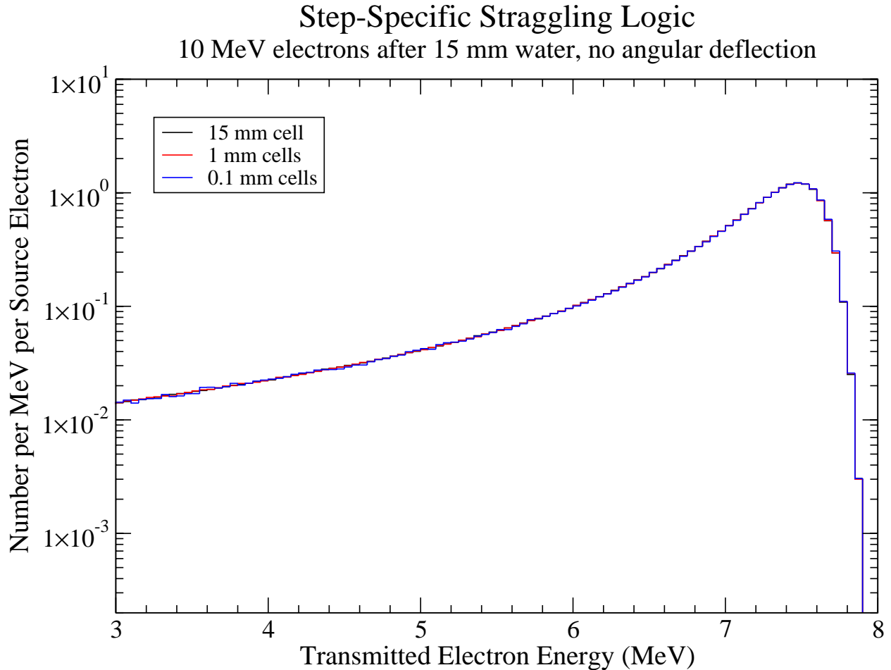
Figure 3. Results of the new step-specific straggling logic for three equivalent geometries now showing the elimination of unphysical step-size artifacts.
