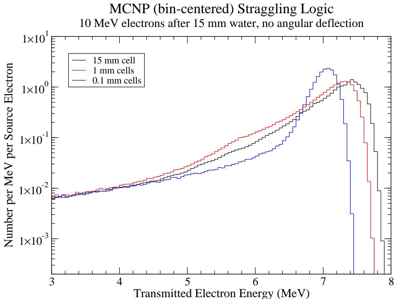
Figure 1. Results of the bin-centered straggling logic for three equivalent geometries showing unphysical step-size artifacts.
