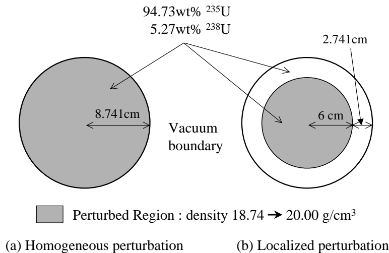
Figure 1. Godiva Geometry and Perturbed Regions
