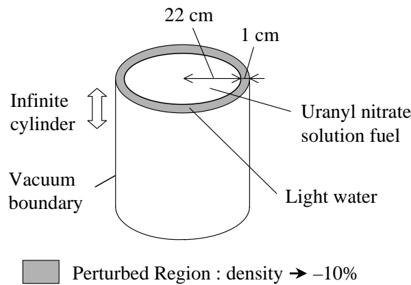
Figure 2. Geometry for the Simplified STACY Model
