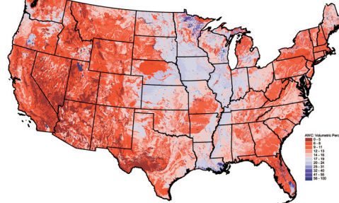
Available Water Holding Capacity (AWC) Map based on Soil Texture
