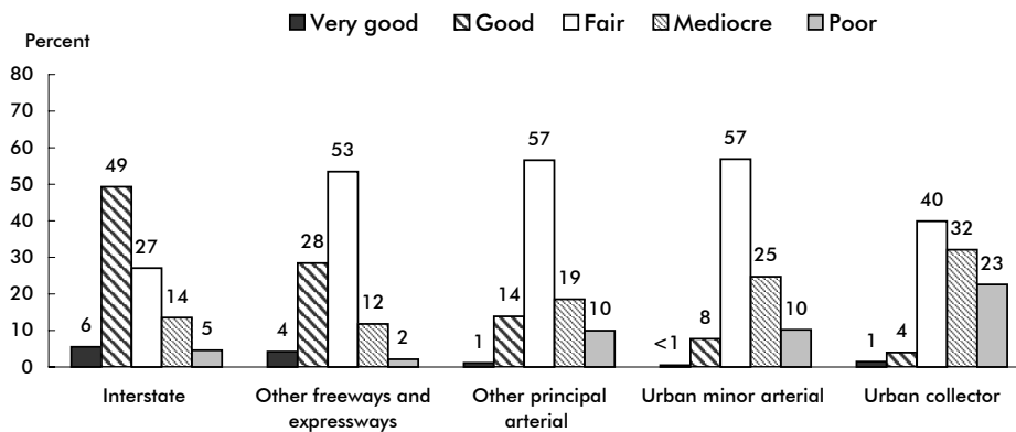
Figure 1-2: Urban Road Conditions in Pennsylvania: 2000
