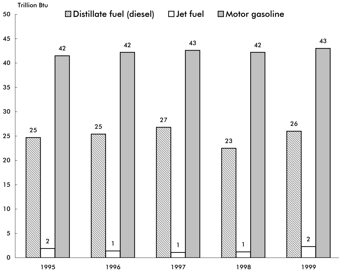
Figure 7-2: North Dakota Transportation Energy Consumption
