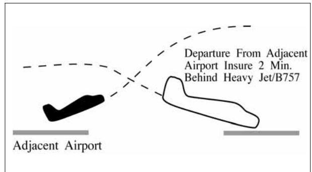
FIG 6-1-2 Adjacent Airport Operation -- Departure
