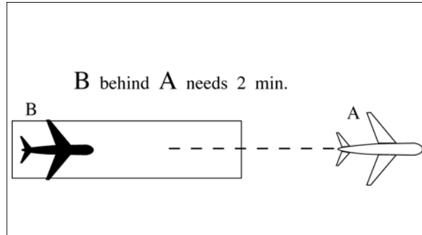
FIG 3-9-4 2 Minute Separation
