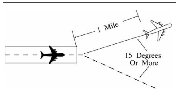
Successive Departures
