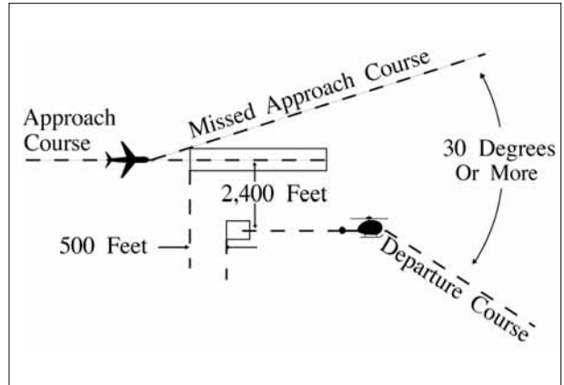
FIG 5-8-12 Parallel Thresholds are Staggered
