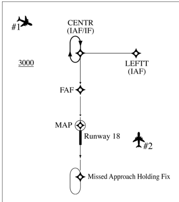
FIG 4-8-2 Approach Clearance Example For RNAV Aircraft
