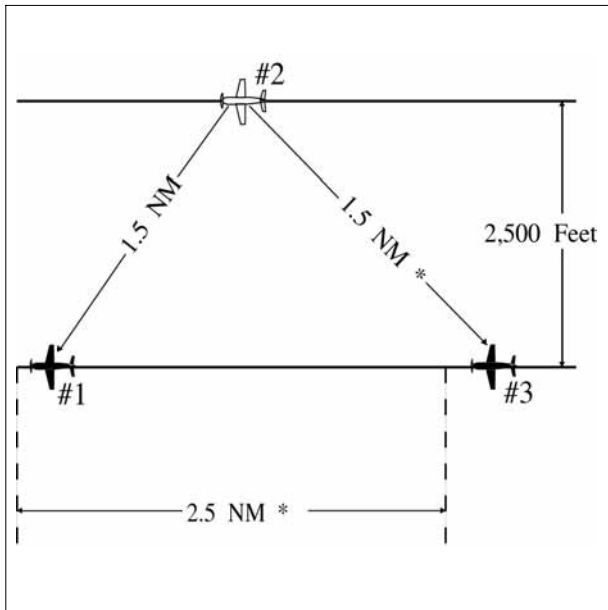
Parallel Dependent ILS/MLS Approaches
