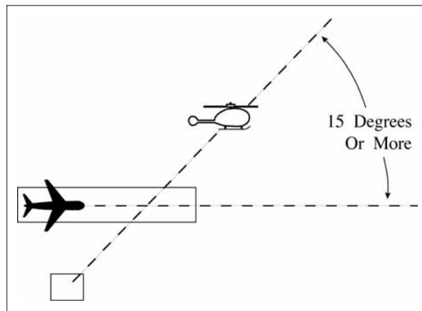
FIG 5-8-6 Intersecting Helicopter Course Departures
