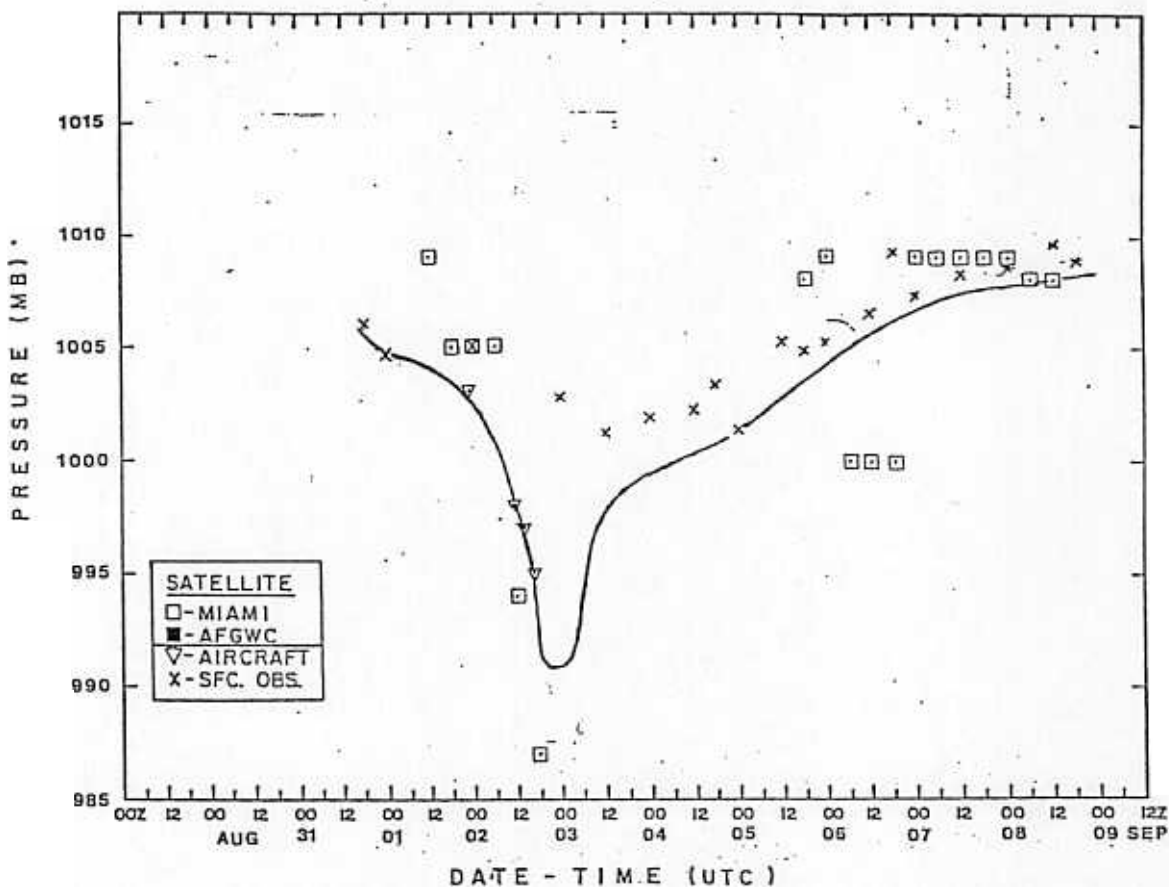
Fig. 2 Best track minimum central pressure curve for Hurricane Debby, 31 August-8 September, 1988.
