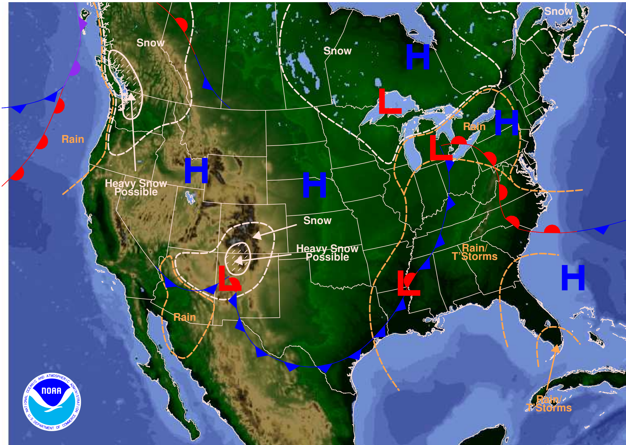
Weather Forecast for Sun, Jan 04, 2009, issued 3:27 AM EST DOC/NOAA/NWS/NCEP/Hydrometeorological Prediction Center Prepared by Gerhardt based on HPC, SPC, and TPC forecasts
