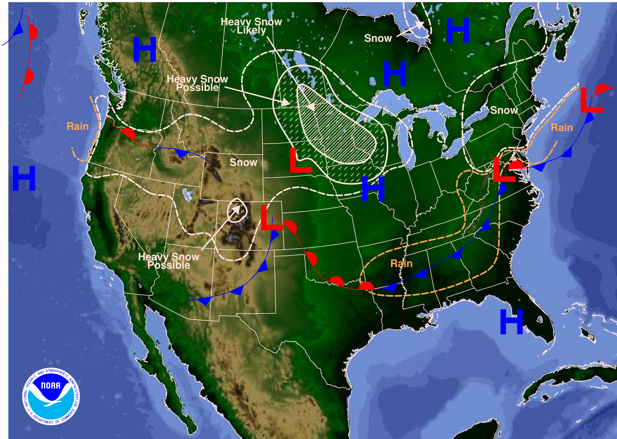
Weather Forecast for Fri, Dec 19, 2008, issued 3:11 PM EST DOC/NOAA/NWS/NCEP/Hydrometeorological Prediction Center Prepared by Kost based on HPC, SPC, and TPC forecasts
