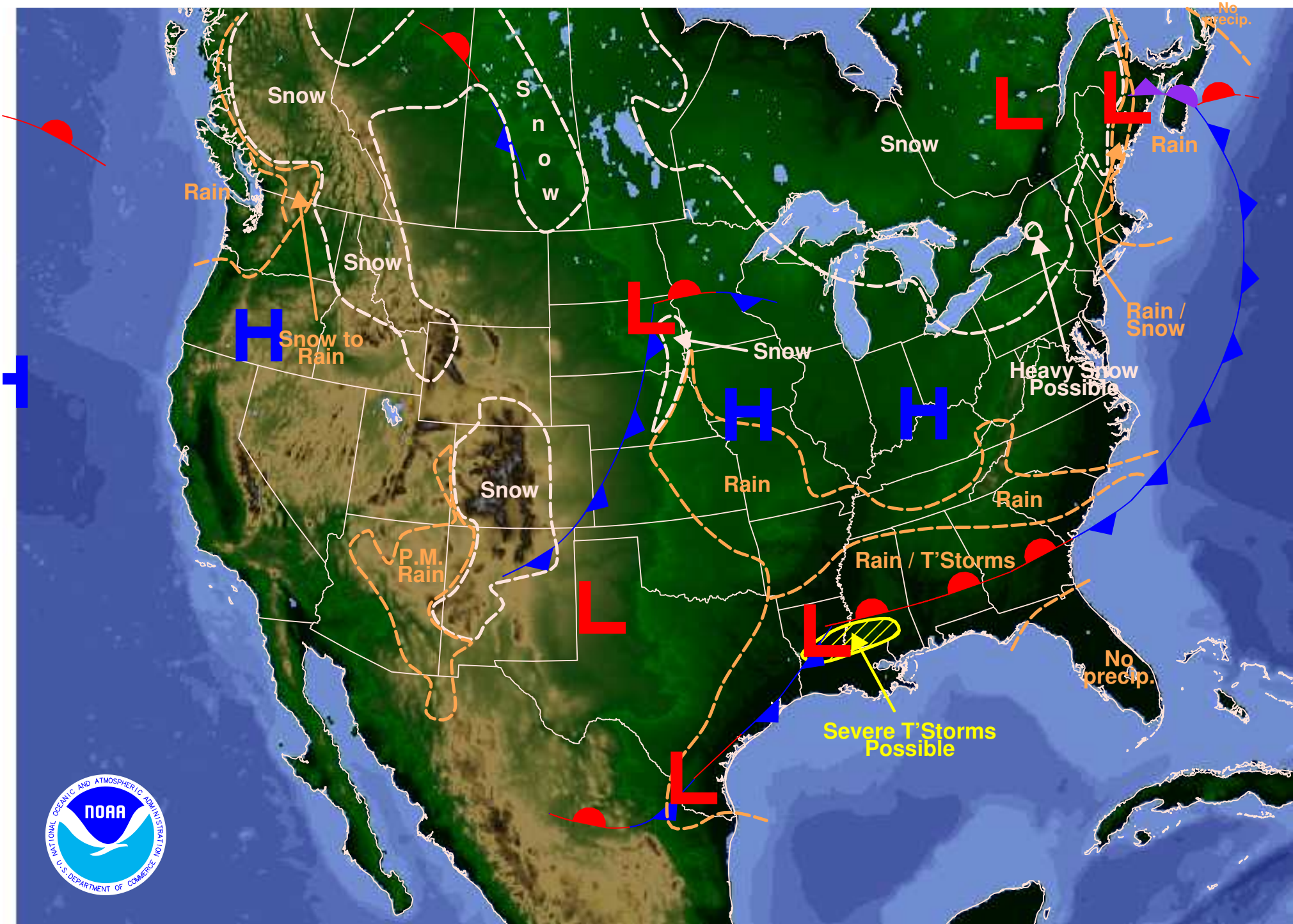
Weather Forecast for Fri, Nov 28, 2008, issued 3:35 PM EST DOC/NOAA/NWS/NCEP/Hydrometeorological Prediction Center Prepared by Kong based on HPC, SPC, and TPC forecasts
