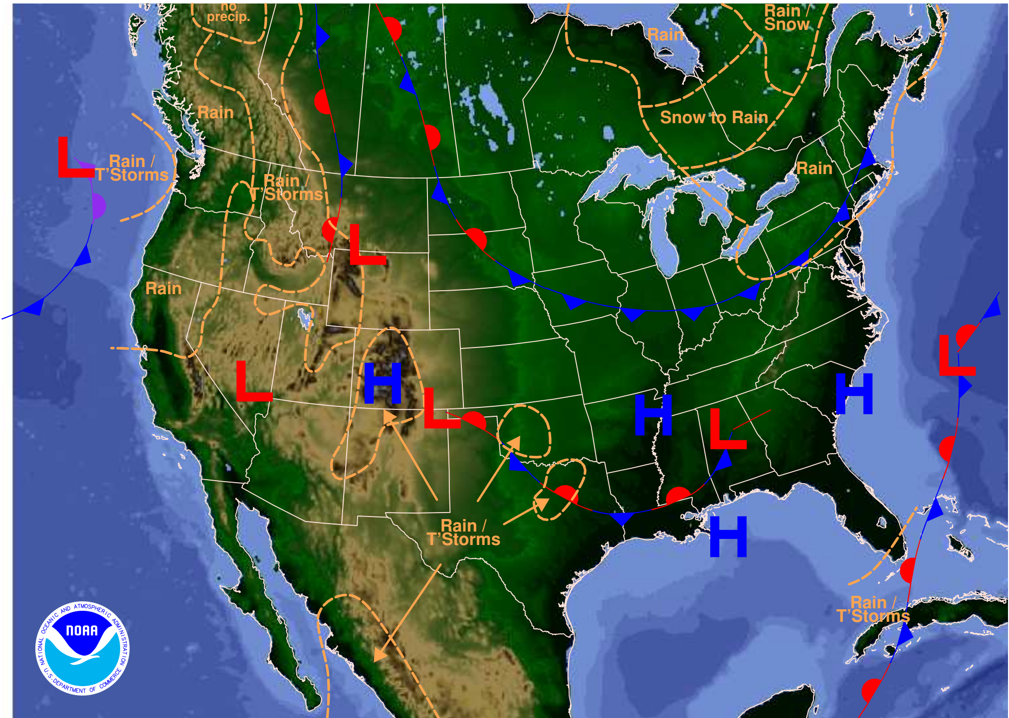
Weather Forecast for Friday, October 03, 2008 DOC/NOAA/NWS/NCEP/Hydrometeorological Prediction Center Prepared by Kong based on HPC, SPC, and TPC forecasts.
