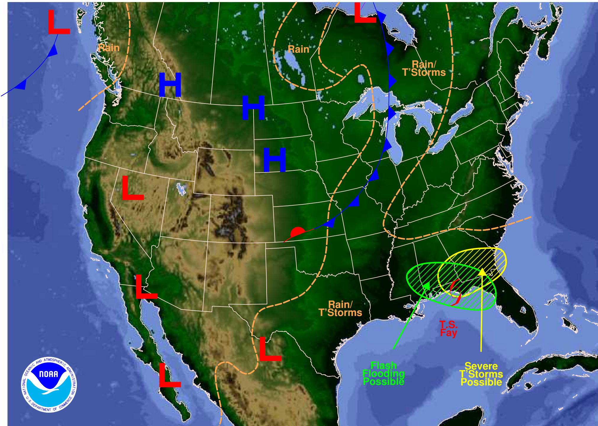
Weather Forecast for Saturday, August 23, 2008 DOC/NOAA/NWS/NCEP/Hydrometeorological Prediction Center Prepared by Fracasso based on HPC, SPC, and TPC forecasts.
