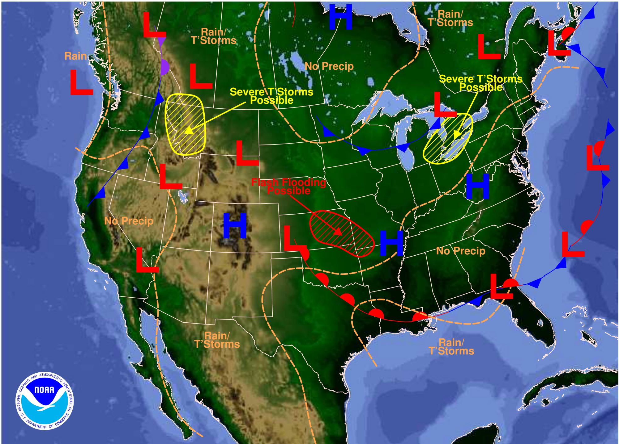
Weather Forecast for Saturday, August 09, 2008 DOC/NOAA/NWS/NCEP/Hydrometeorological Prediction Center Prepared by Kost based on HPC, SPC, and TPC forecasts.
