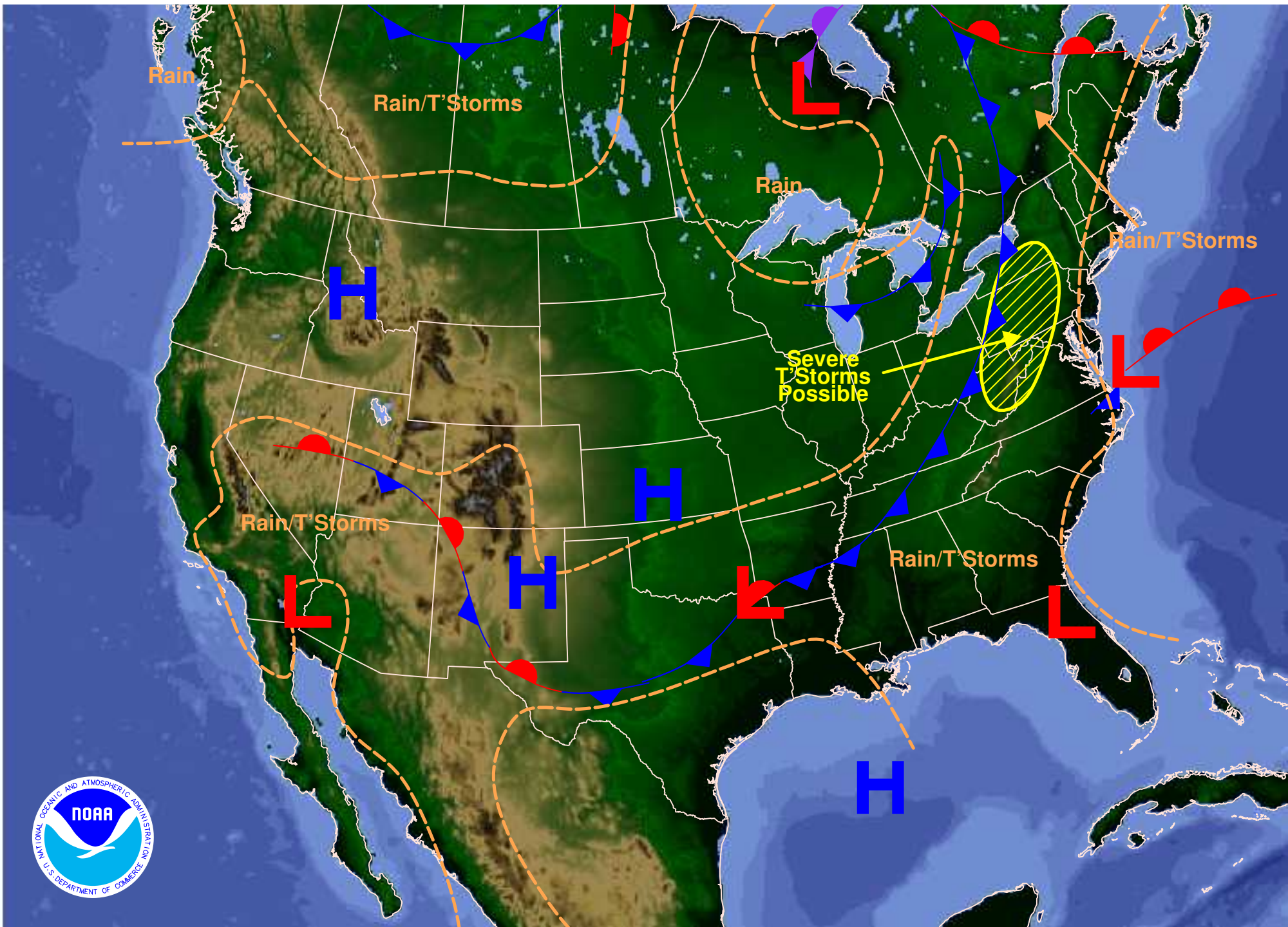
Weather Forecast for Sunday, July 13, 2008 DOC/NOAA/NWS/NCEP/Hydrometeorological Prediction Center Prepared by Engelman based on HPC, SPC, and TPC forecasts.
