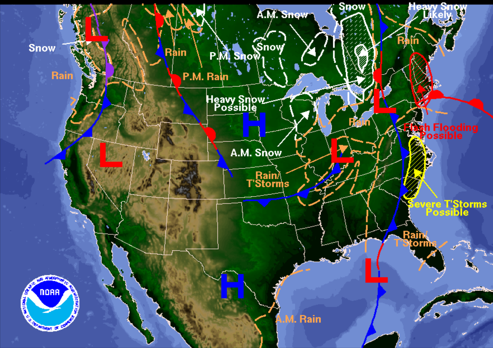
Weather Forecast for Monday, April 28, 2008 DOC/NOAA/NWS/NCEP/Hydrometeorological Prediction Center Prepared by Rubin-Oster based on HPC, SPC, and TPC forecasts.
