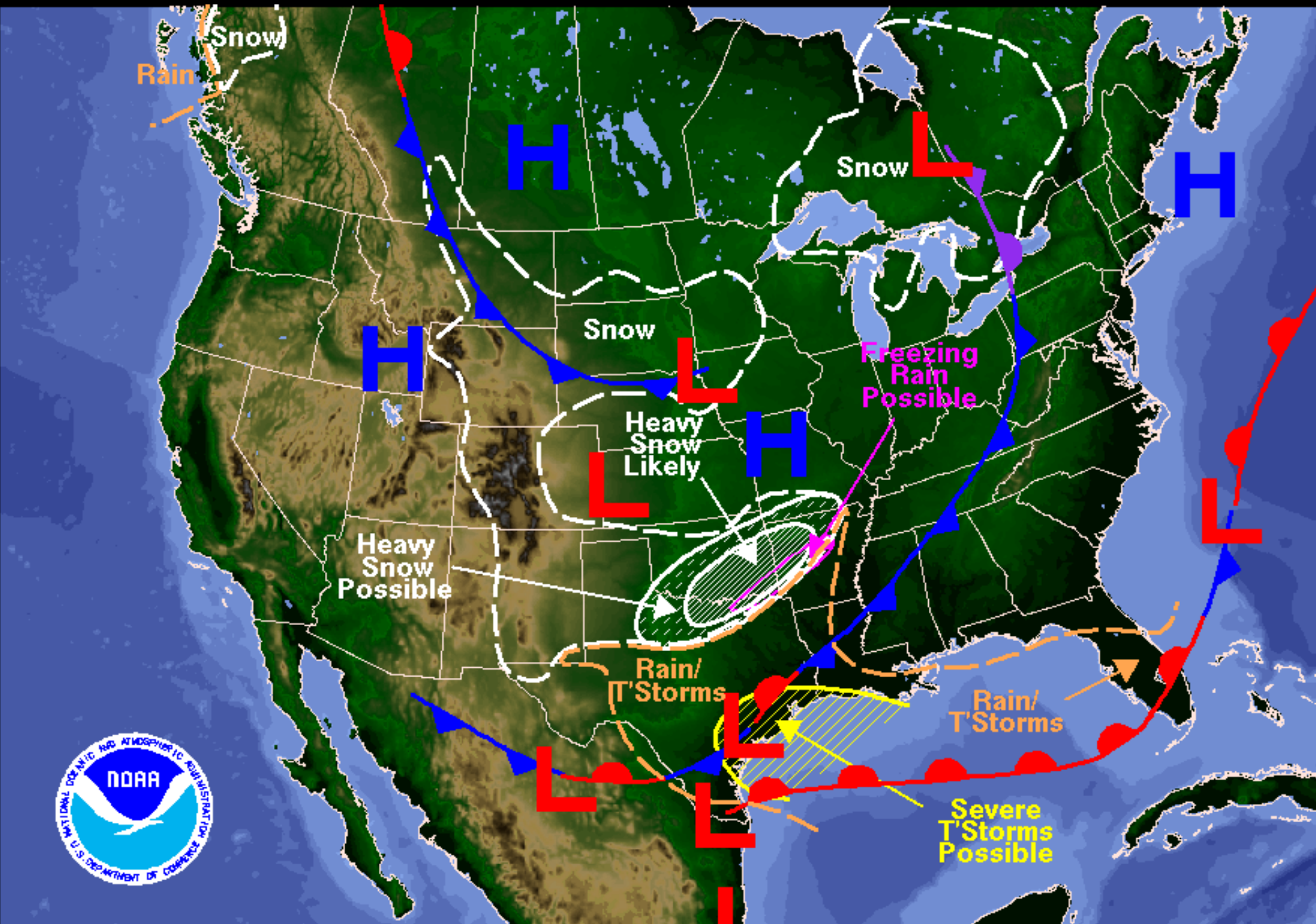
Weather Forecast for Thursday, March 06, 2008 DOC/NOAA/NWS/NCEP/Hydrometeorological Prediction Center Prepared by Fracasso based on HPC, SPC, and TPC forecasts.
