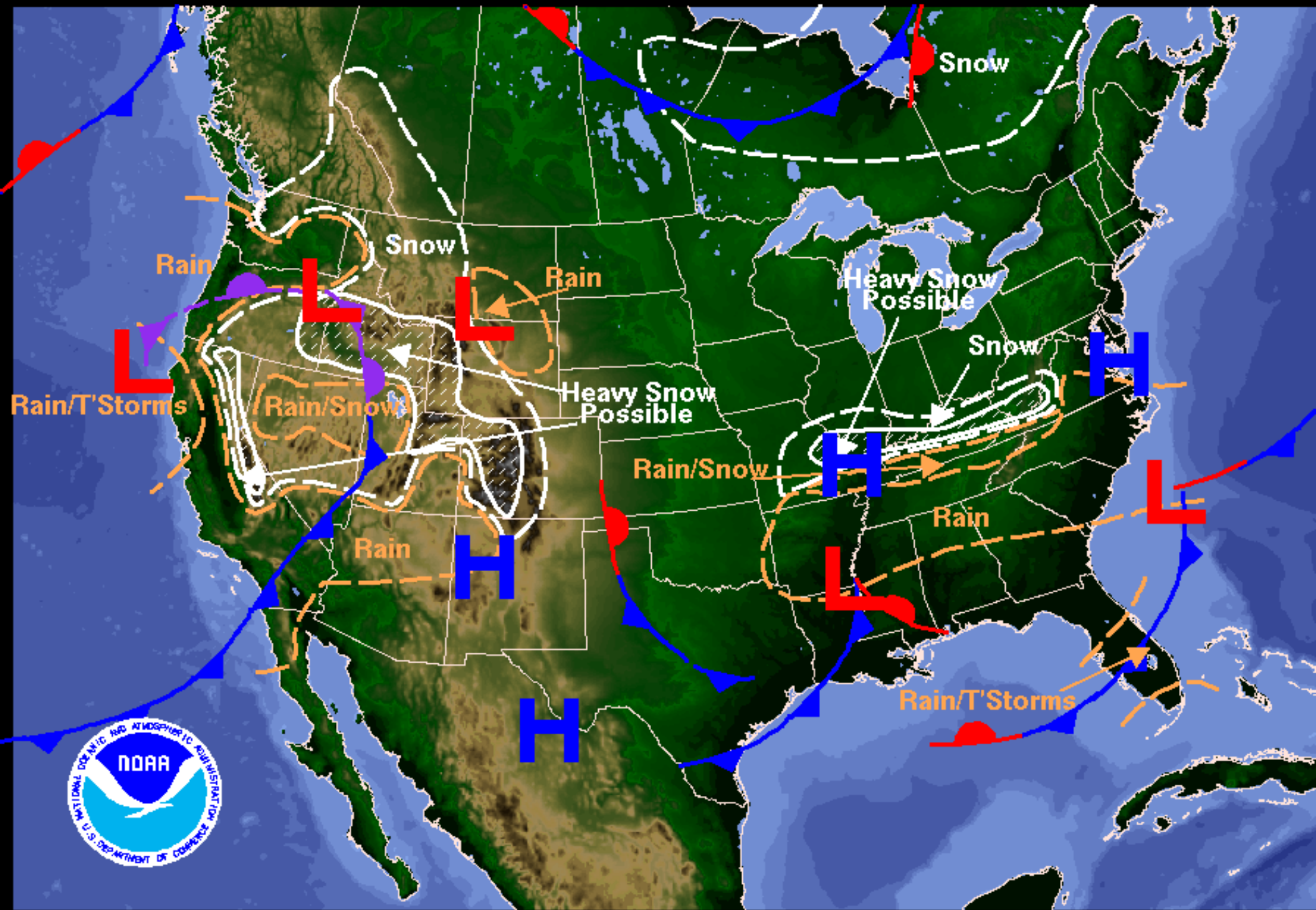
Weather Forecast for Sunday, February 24, 2008 DOC/NOAA/NWS/NCEP/Hydrometeorological Prediction Center Prepared by Engelman based on HPC, SPC, and TPC forecasts.
