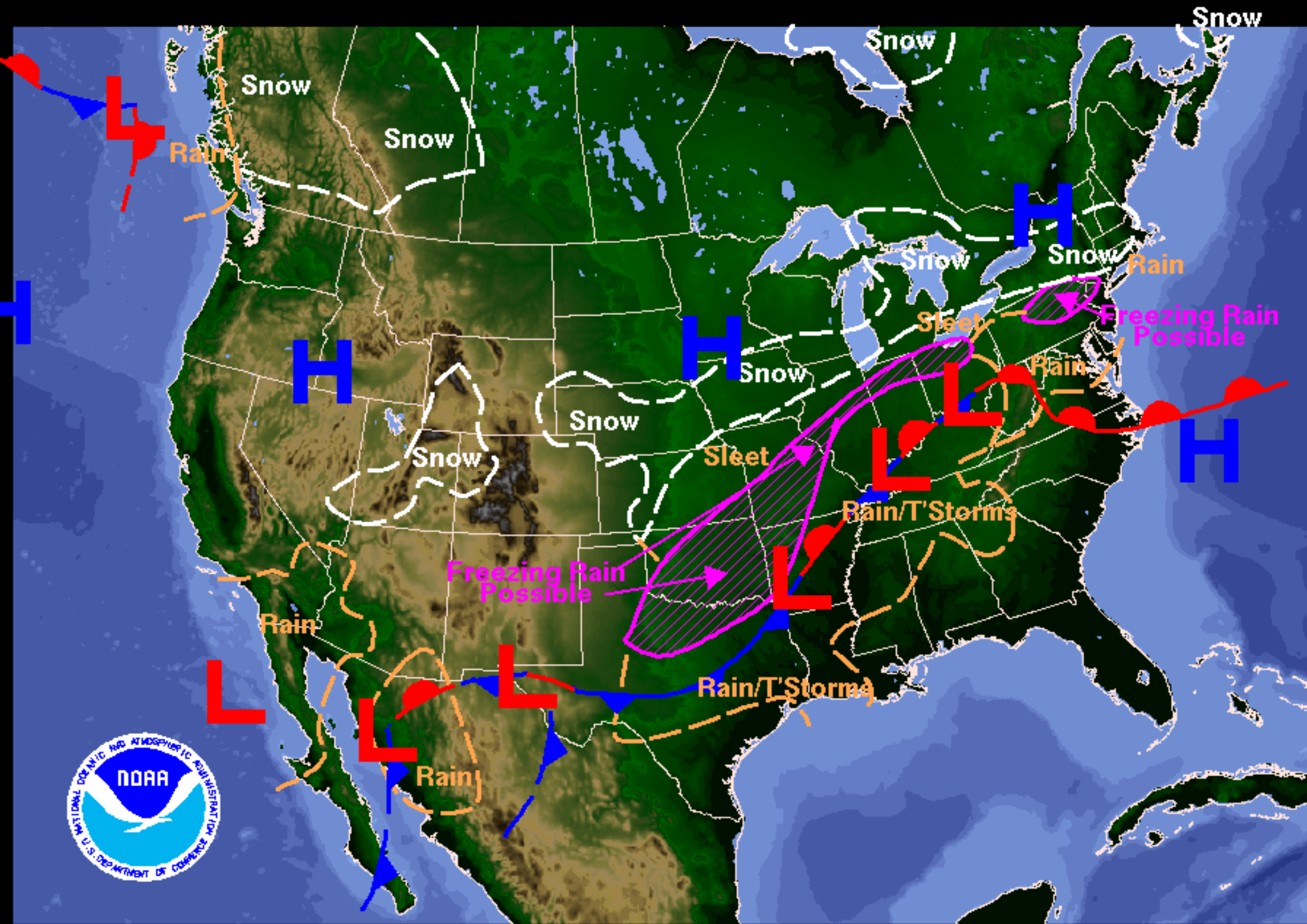
Weather Forecast for Sunday, December 09, 2007 DOC/NOAA/NWS/NCEP/Hydrometeorological Prediction Center Prepared by Kocin based on HPC, SPC, and TPC forecasts.
