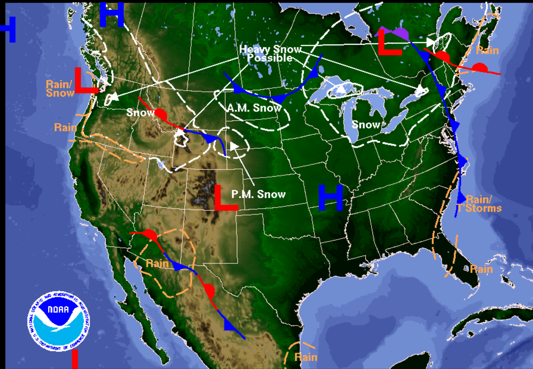
Weather Forecast for Thursday, November 29, 2007 DOC/NOAA/NWS/NCEP/Hydrometeorological Prediction Center Prepared by Rubin-Oster based on HPC, SPC, and TPC forecasts.
