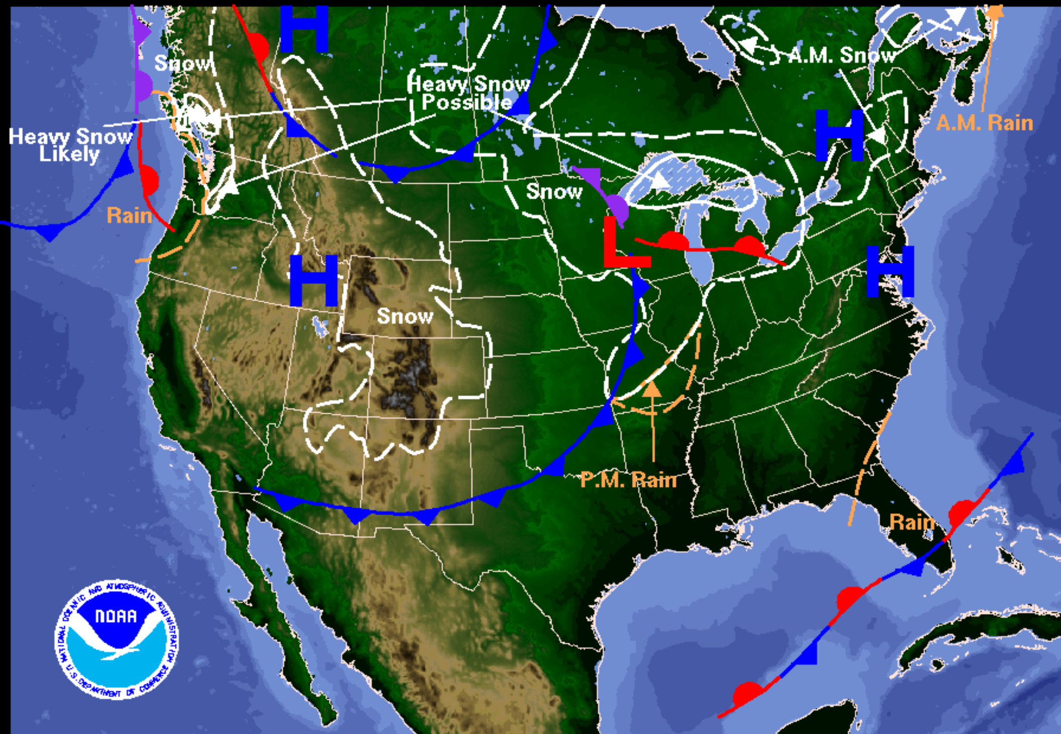
Weather Forecast for Wednesday, November 28, 2007 DOC/NOAA/NWS/NCEP/Hydrometeorological Prediction Center Prepared by Rubin-Oster based on HPC, SPC, and TPC forecasts.
