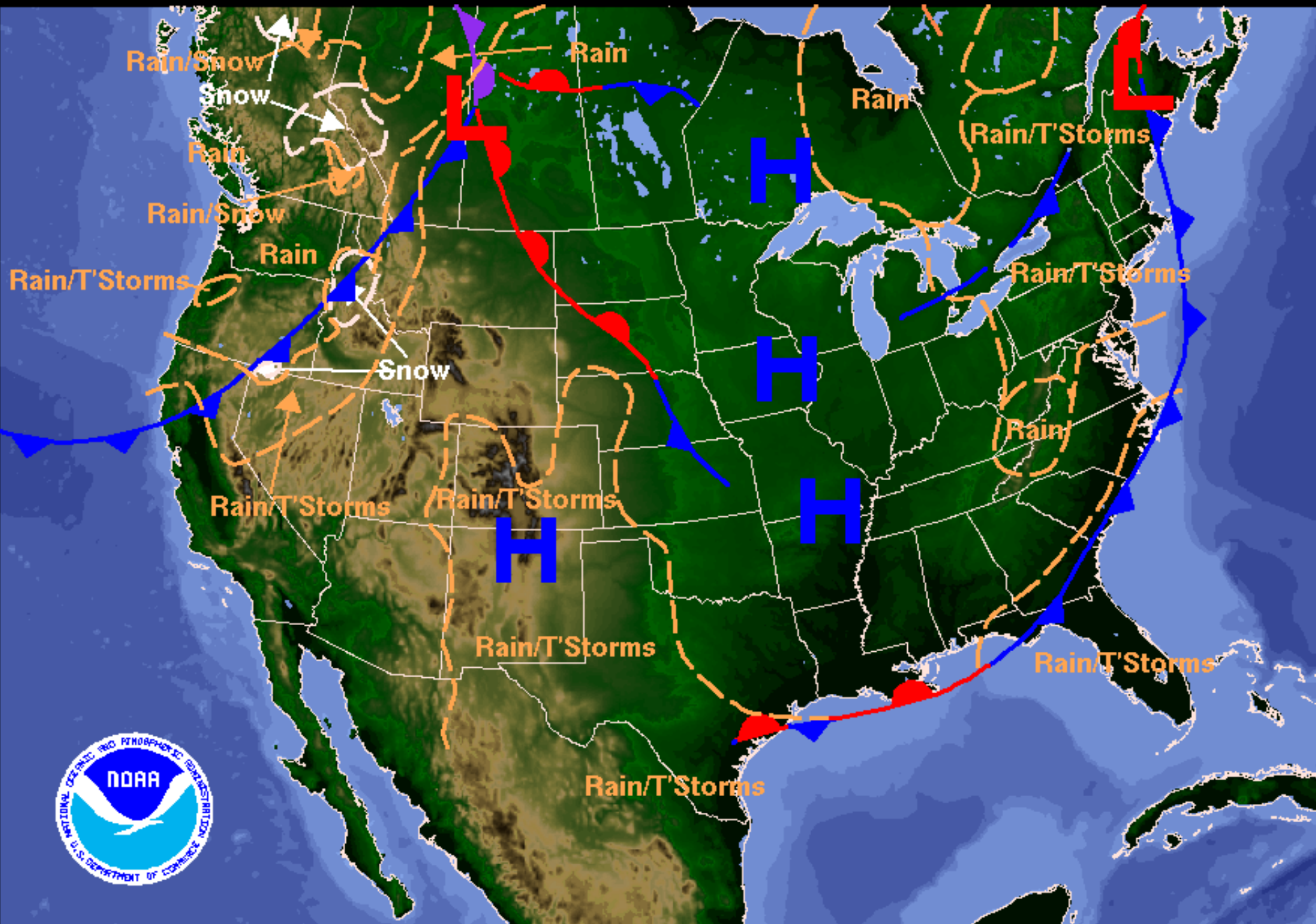
Weather Forecast for Friday, September 28, 2007 DOC/NOAA/NWS/NCEP/Hydrometeorological Prediction Center Prepared by Kocin based on HPC, SPC, and TPC forecasts.
