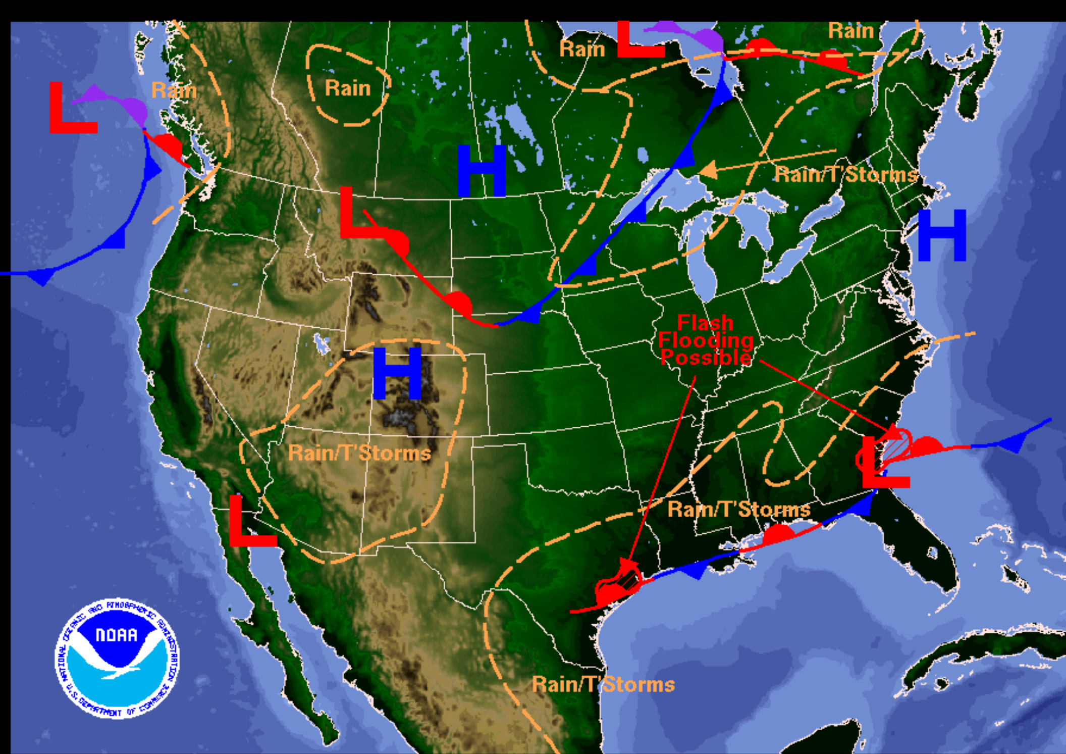
Weather Forecast for Sunday, September 02, 2007 DOC/NOAA/NWS/NCEP/Hydrometeorological Prediction Center Prepared by Otto based on HPC, SPC, and TPC forecasts.
