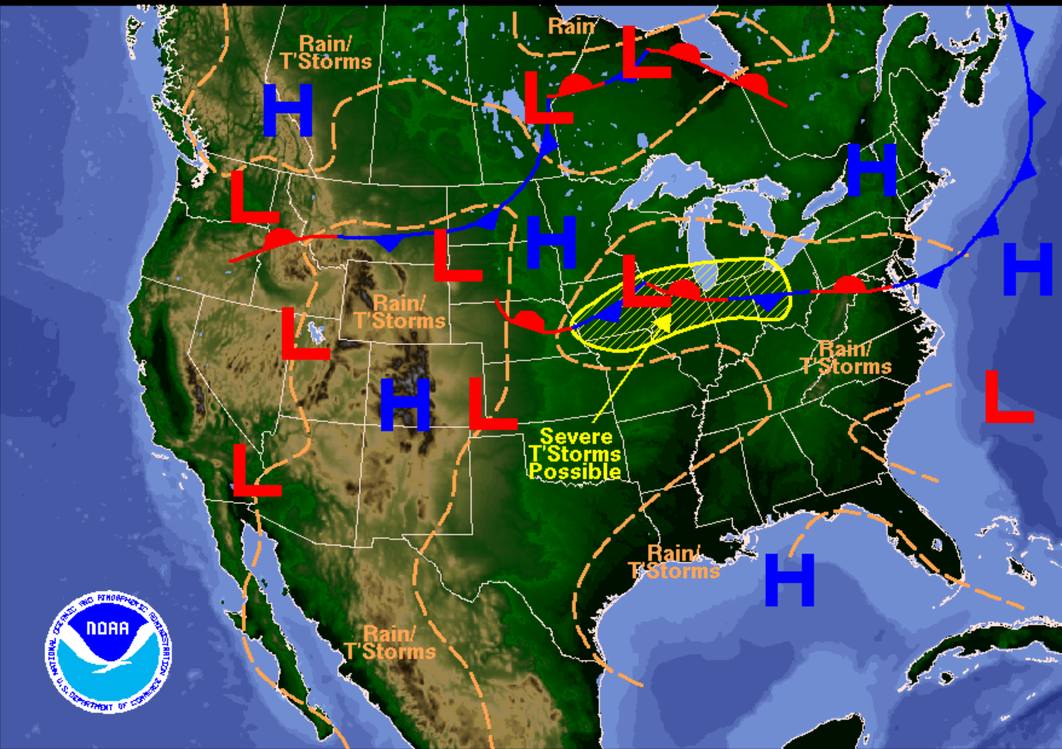
Weather Forecast for Sunday, August 05, 2007 DOC/NOAA/NWS/NCEP/Hydrometeorological Prediction Center Prepared by Fracasso based on HPC, SPC, and TPC forecasts.
