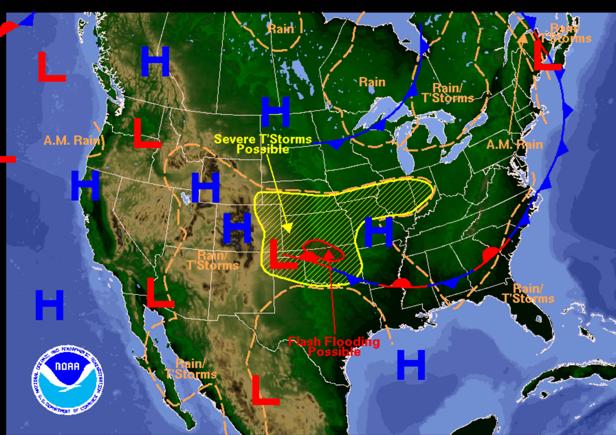
Weather Forecast for Thursday, July 12, 2007 DOC/NOAA/NWS/NCEP/Hydrometeorological Prediction Center Prepared by Rubin-Oster based on HPC, SPC, and TPC forecasts.
