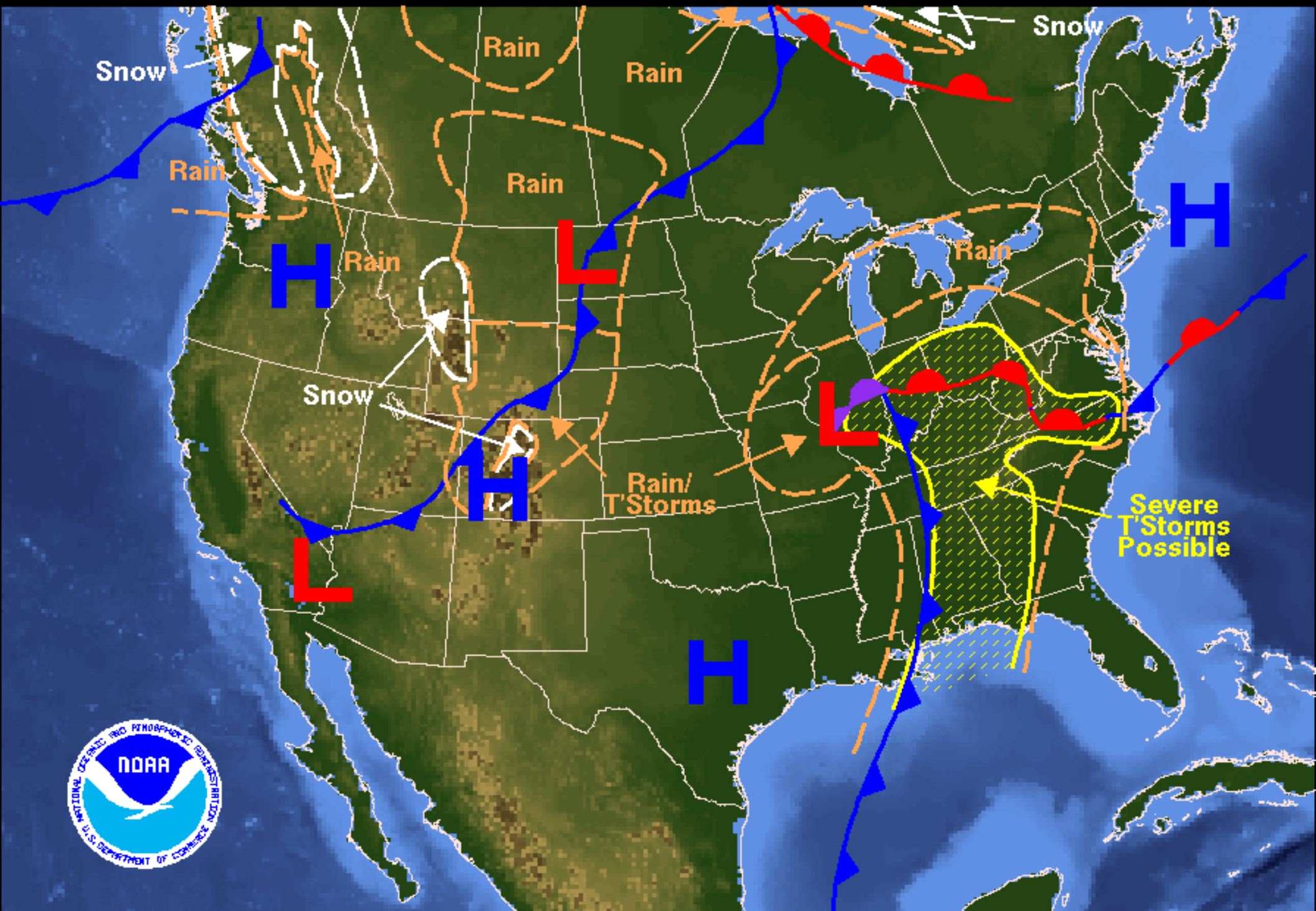
Weather Forecast for Thursday, April 26, 2007 DOC/NOAA/NWS/NCEP/Hydrometeorological Prediction Center Prepared by Fracasso based on HPC, SPC, and TPC forecasts.
