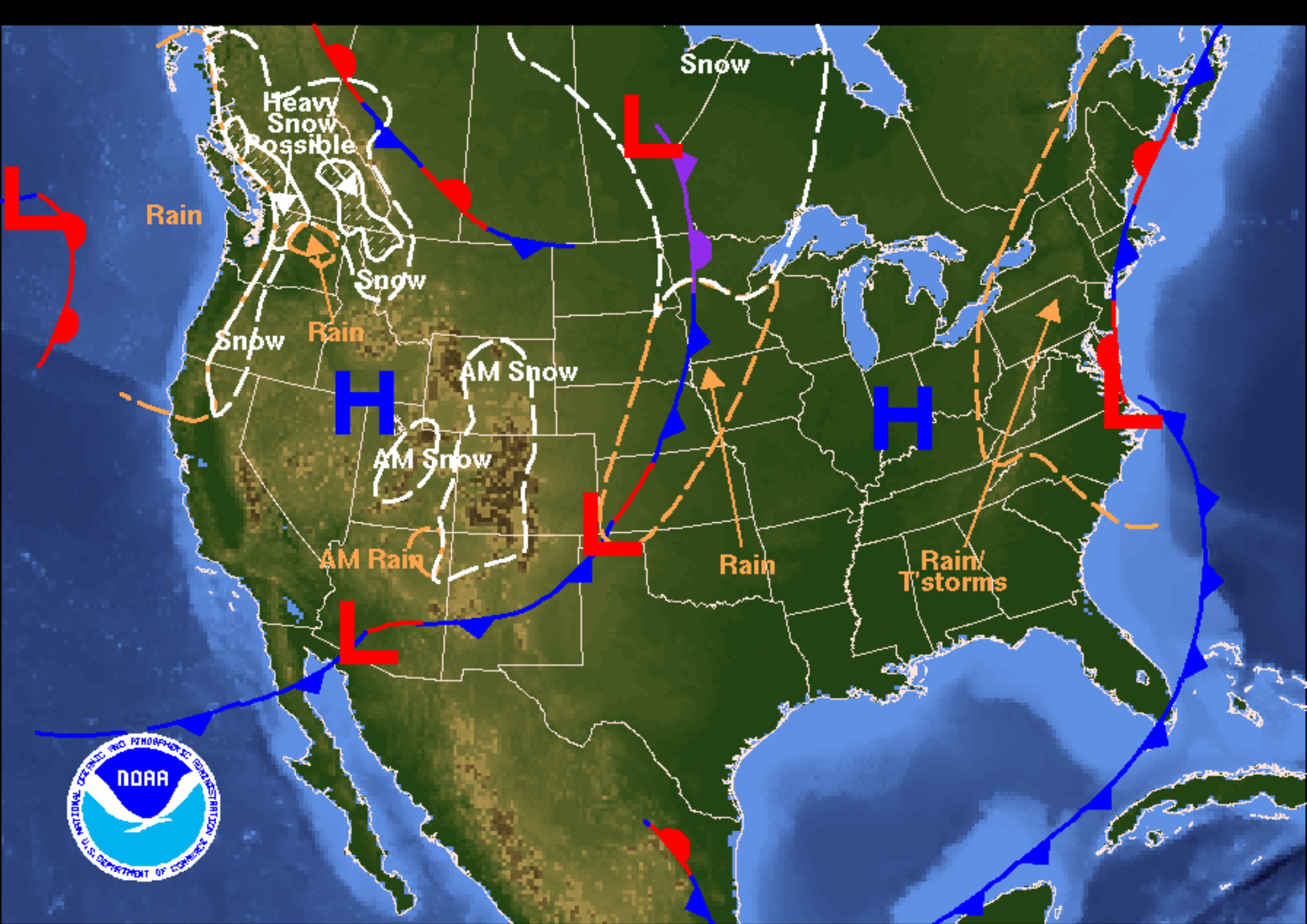
Weather Forecast for Sunday, November 12, 2006 DOC/NOAA/NWS/NCEP/Hydrometeorological Prediction Center Prepared by Orrison based on HPC, SPC, and TPC forecasts.
