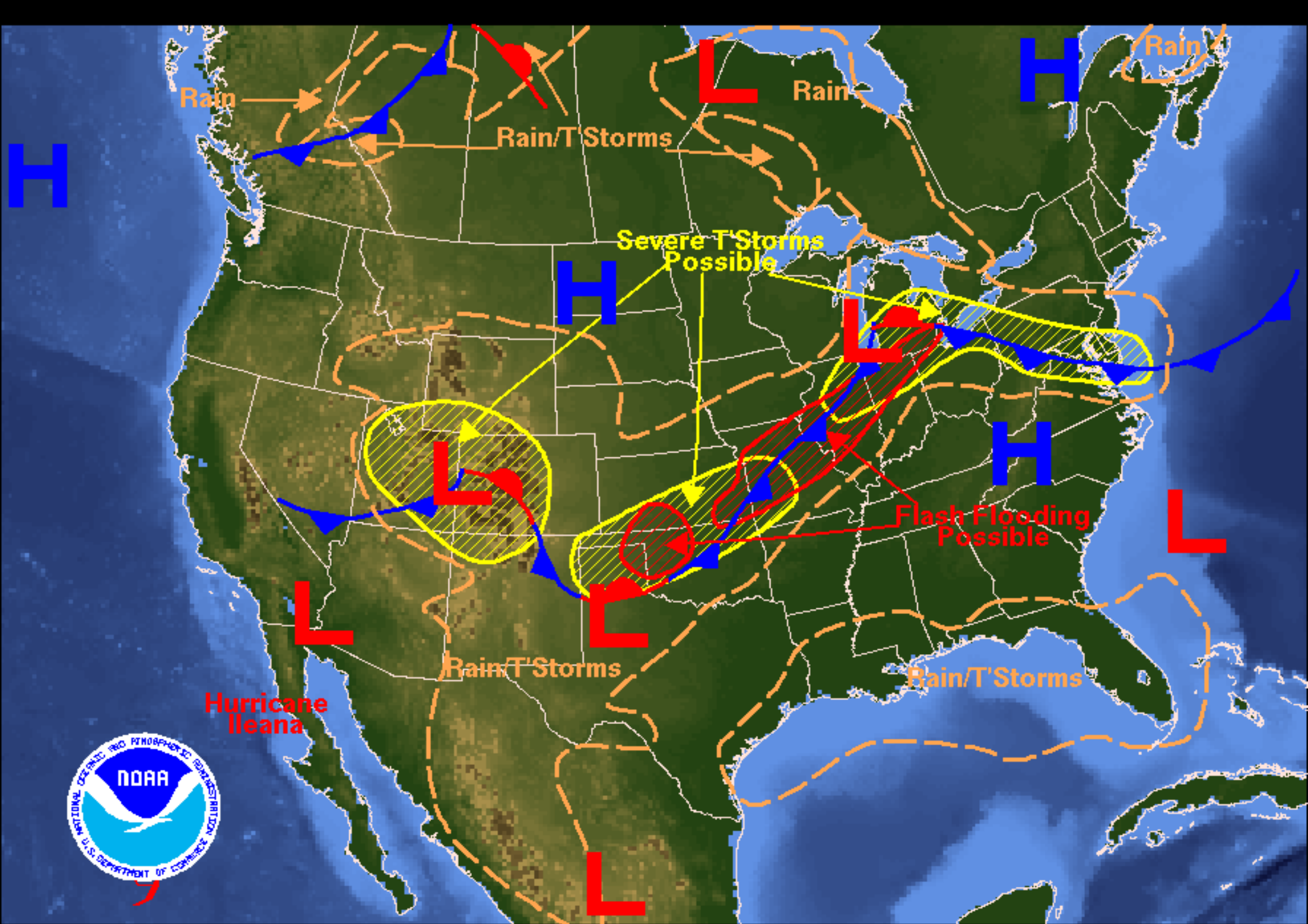
Weather Forecast for Saturday, August 26, 2006 DOC/NOAA/NWS/NCEP/Hydrometeorological Prediction Center Prepared by Rubin-Oster based on HPC, SPC, and TPC forecasts.
