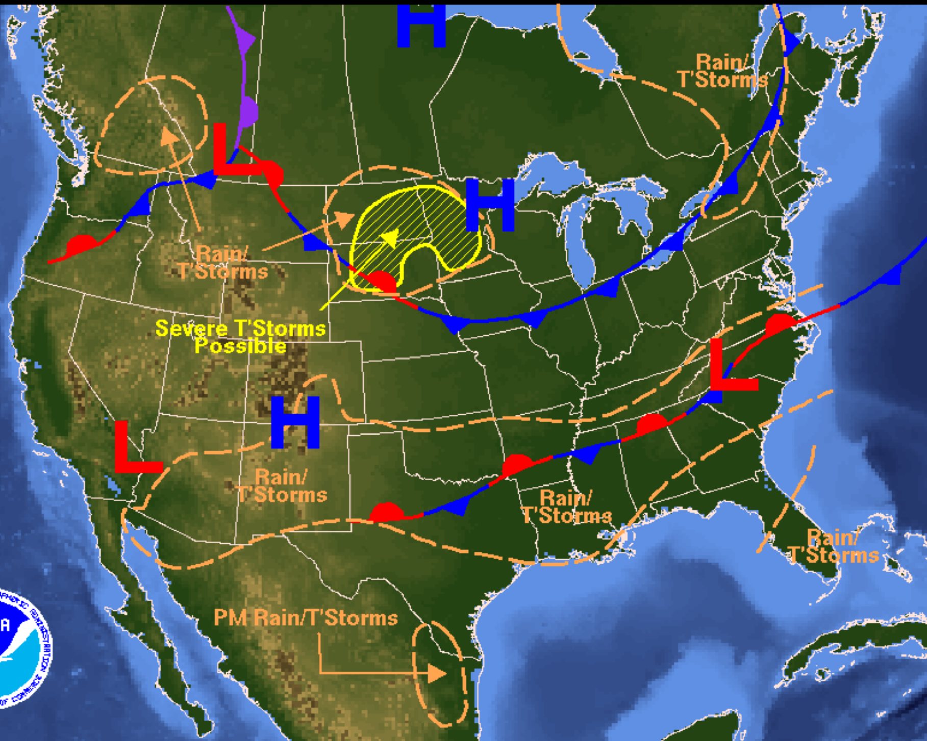
Weather Forecast for Tuesday, August 22, 2006 DOC/NOAA/NWS/NCEP/Hydrometeorological Prediction Center Prepared by Szatanek based on HPC, SPC, and TPC forecasts.
