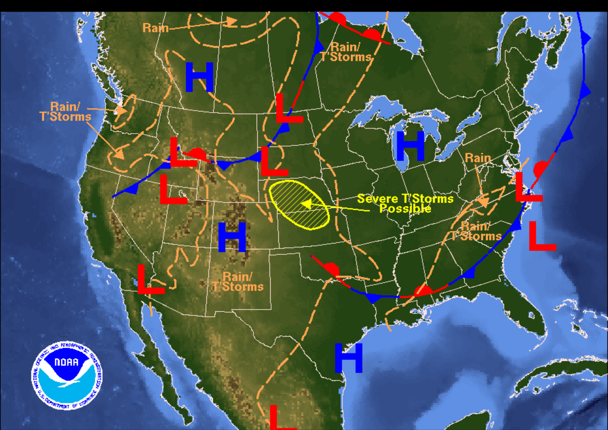
Weather Forecast for Wednesday, August 16, 2006 DOC/NOAA/NWS/NCEP/Hydrometeorological Prediction Center Prepared by Rubin-Oster/Otto based on HPC, SPC, and TPC forecasts.
