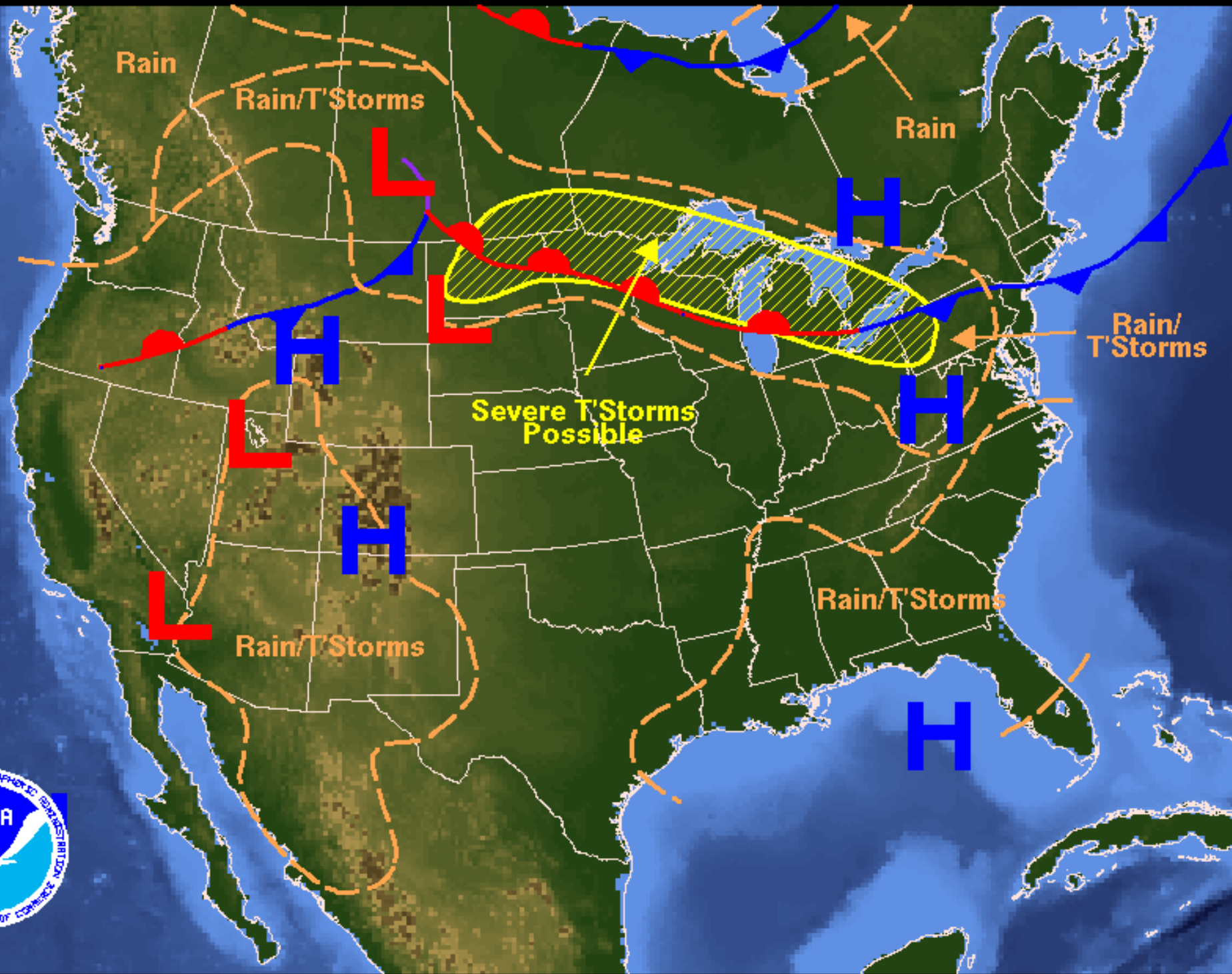
Weather Forecast for Sunday, July 30, 2006 DOC/NOAA/NWS/NCEP/Hydrometeorological Prediction Center Prepared by Scheck based on HPC, SPC, and TPC forecasts.
