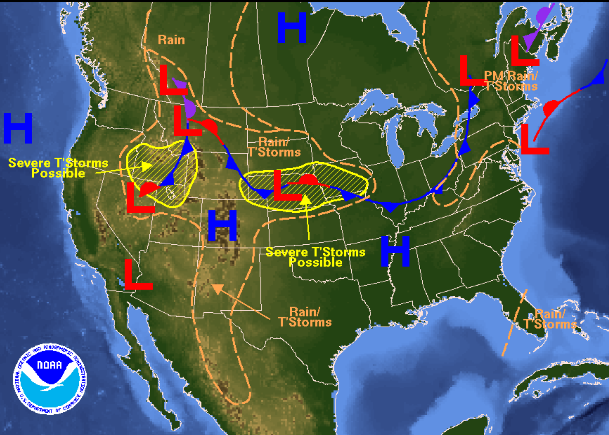
Weather Forecast for Friday, June 09, 2006 DOC/NOAA/NWS/NCEP/Hydrometeorological Prediction Center Prepared by Szatanek based on HPC, SPC, and TPC forecasts.
