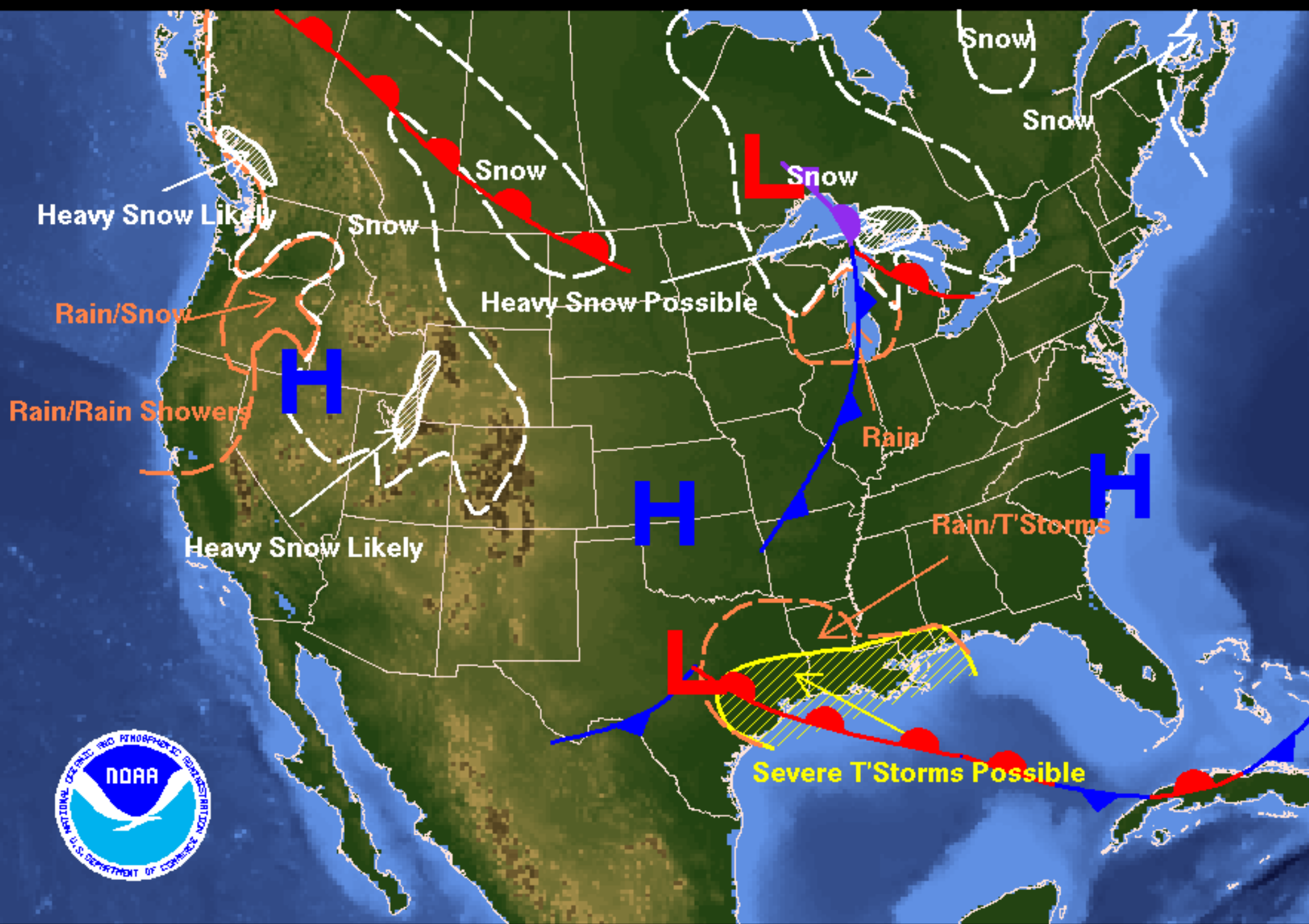
Weather Forecast for Wednesday, February 01, 2006 DOC/NOAA/NWS/NCEP/Hydrometeorological Prediction Center Prepared by Kimberlain based on HPC, SPC, and TPC forecasts.
