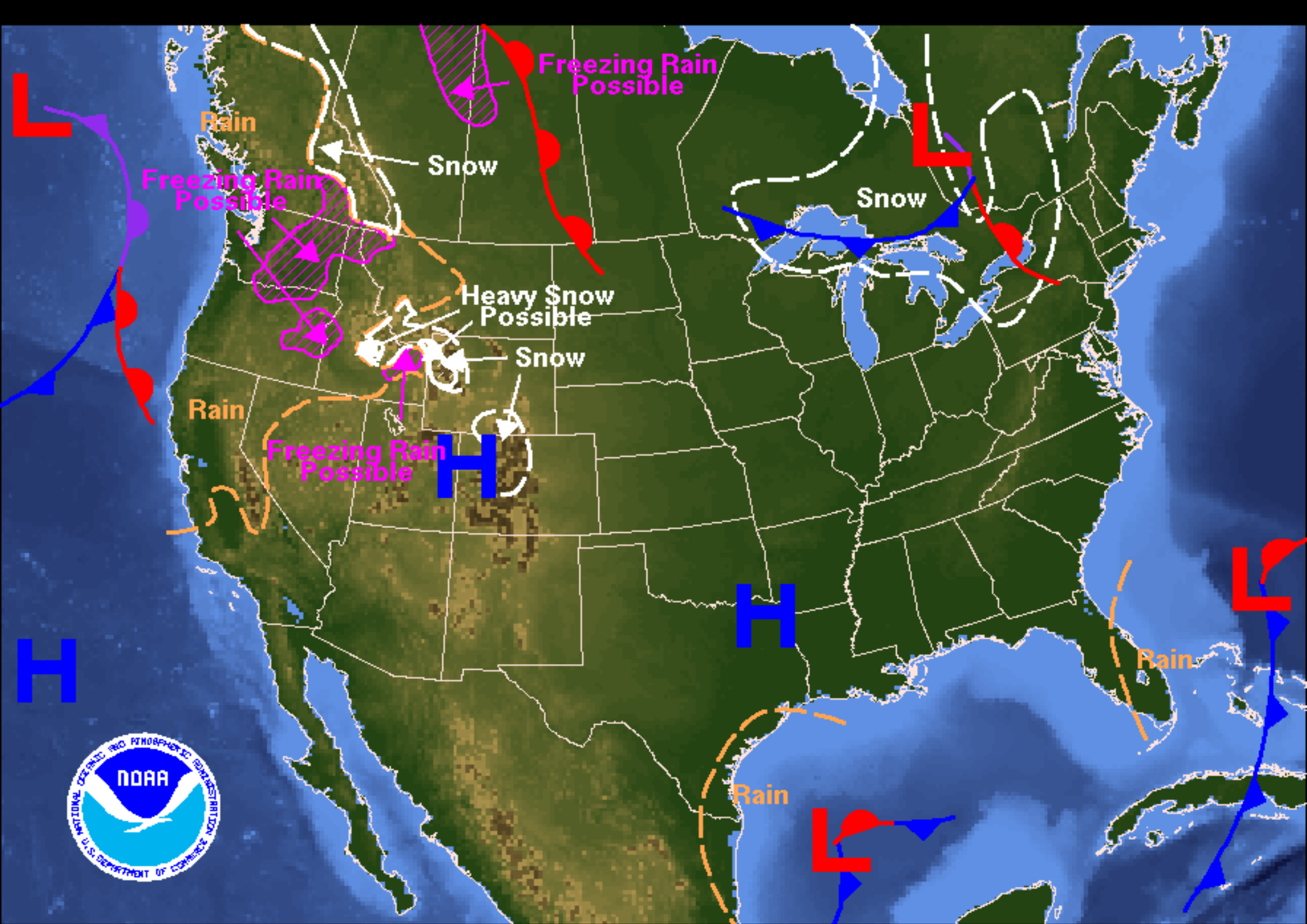
Weather Forecast for Wednesday, December 21, 2005 DOC/NOAA/NWS/NCEP/Hydrometeorological Prediction Center Prepared by Trimarco/Bell based on HPC, SPC, and TPC forecasts.
