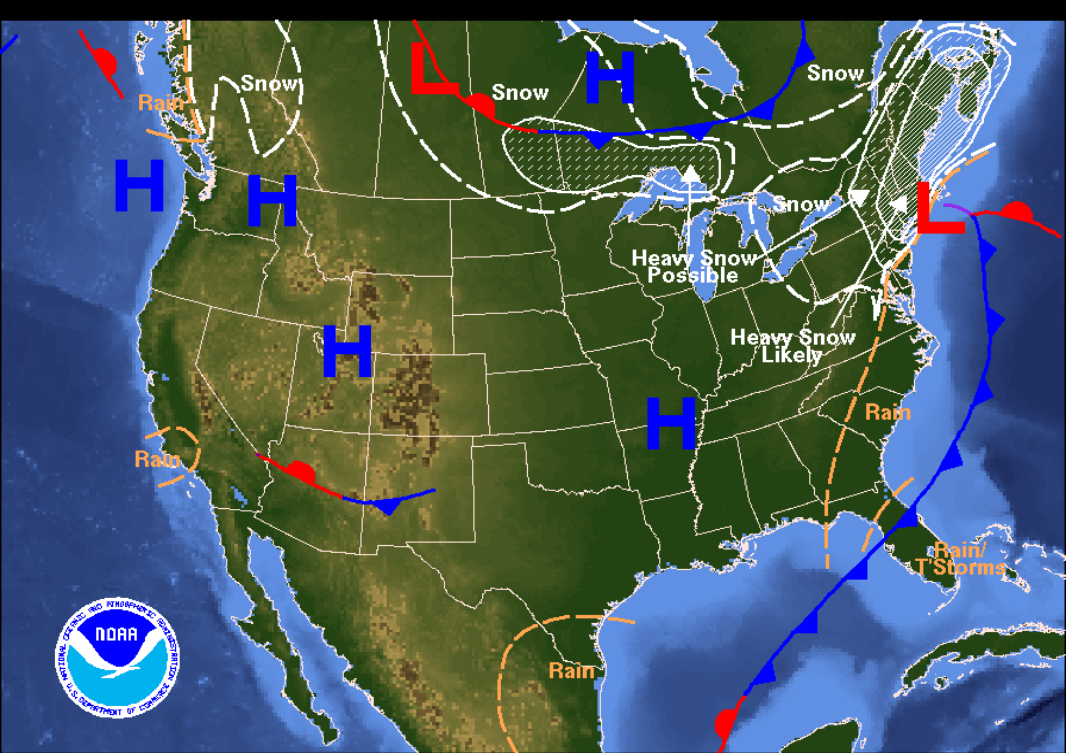
Weather Forecast for Friday, December 09, 2005 DOC/NOAA/NWS/NCEP/Hydrometeorological Prediction Center Prepared by Fries based on HPC, SPC, and TPC forecasts.
